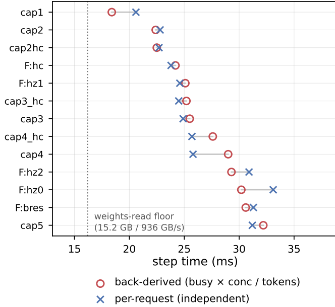
Fig. 3. Per-step cost by two independent measurements, one run per row: circles derive it from busy time, crosses from per-request decode intervals. They agree to within 12% and rank the runs nearly identically ( \rho = 0.967 ). The dotted line is the cost of reading the weights once; every run sits above it.
