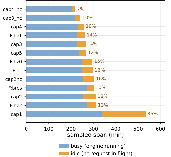
Fig. 2. Wall clock split into busy and idle for every completed run, ordered by total duration. Idle is 7.4% for the fastest configuration and 36.3% for the slowest. Note bres : it cuts idle to 10.1% and is still slower than its own baseline, because busy time grows instead.
