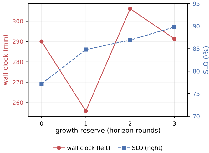
Fig. 5. The growth reserve is not a free parameter. Removing it costs 13.5 pp of SLO; two rounds is 15 minutes slower than three. The optimum at one round touches the static front and does not cross it.
