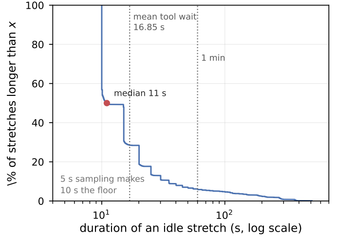
Fig. 4. Survival function of idle-stretch duration, pooled over all completed runs (1,849 stretches). The median stretch is 11 s and 30% exceed 20 s—the same scale as the 16.85 s mean tool wait, and far above the 2 s control cycle. The vertical cliff at 10 s is the sampling floor.
