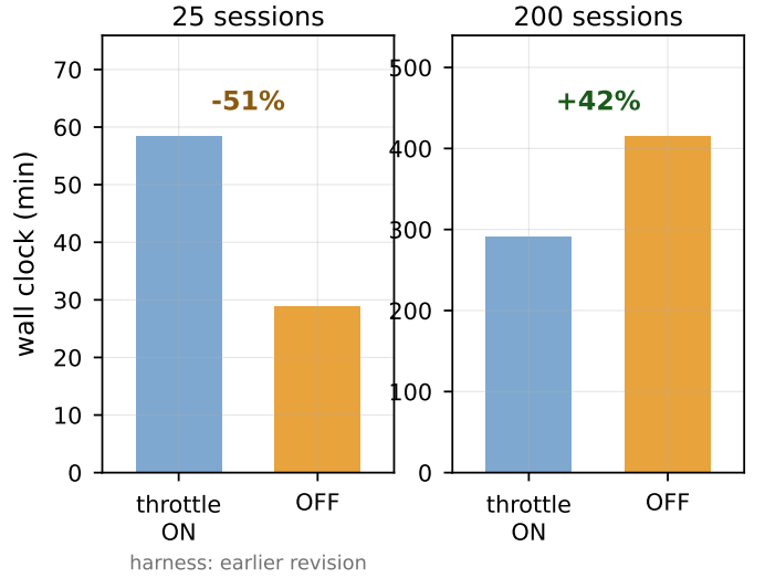
Fig. 6. The same throttle switch, two load tiers, opposite signs. The 25-session bars are from an earlier harness revision and are shown as a direction, not a magnitude; the matching current-harness arm was interrupted and is not reported.
