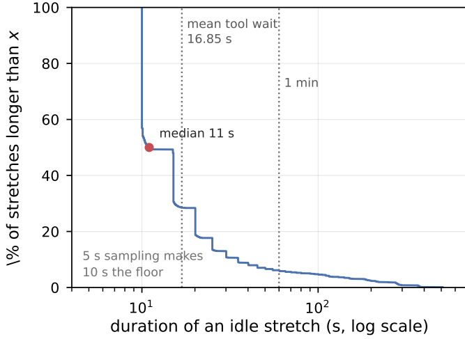
Fig. 4. Survival function of idle-stretch duration, pooled over all completed runs (1,849 stretches). The median stretch is 11 s and 30% exceed 20 s—the same scale as the 16.85 s mean tool wait, and far above the 2 s control cycle. The vertical cliff at 10 s is the sampling floor.
