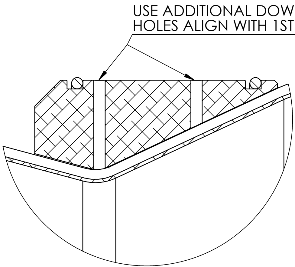
DETAIL B SCALE 1 : 1
