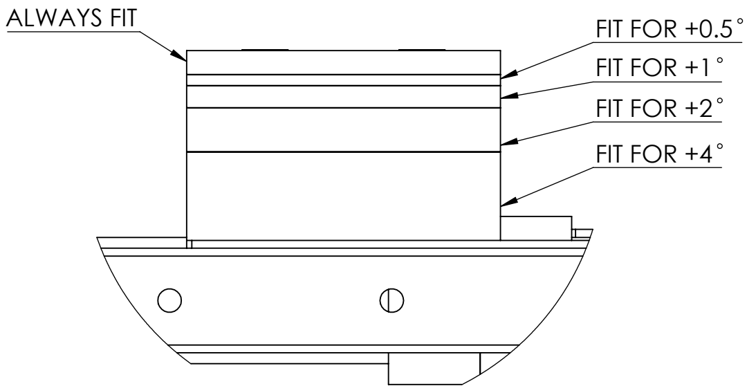
DETAIL A SCALE 1 : 2
