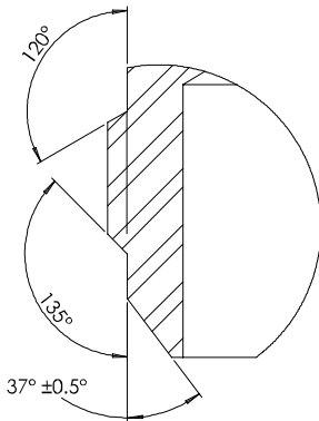
DETAIL D SCALE 3:1
