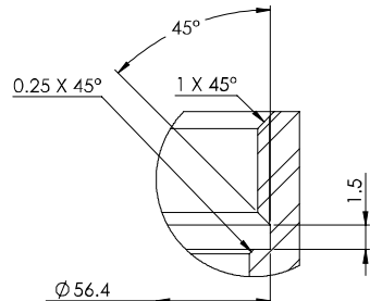
DETAIL D SCALE 4 : 1
