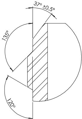
DETAIL B SCALE 3:1
