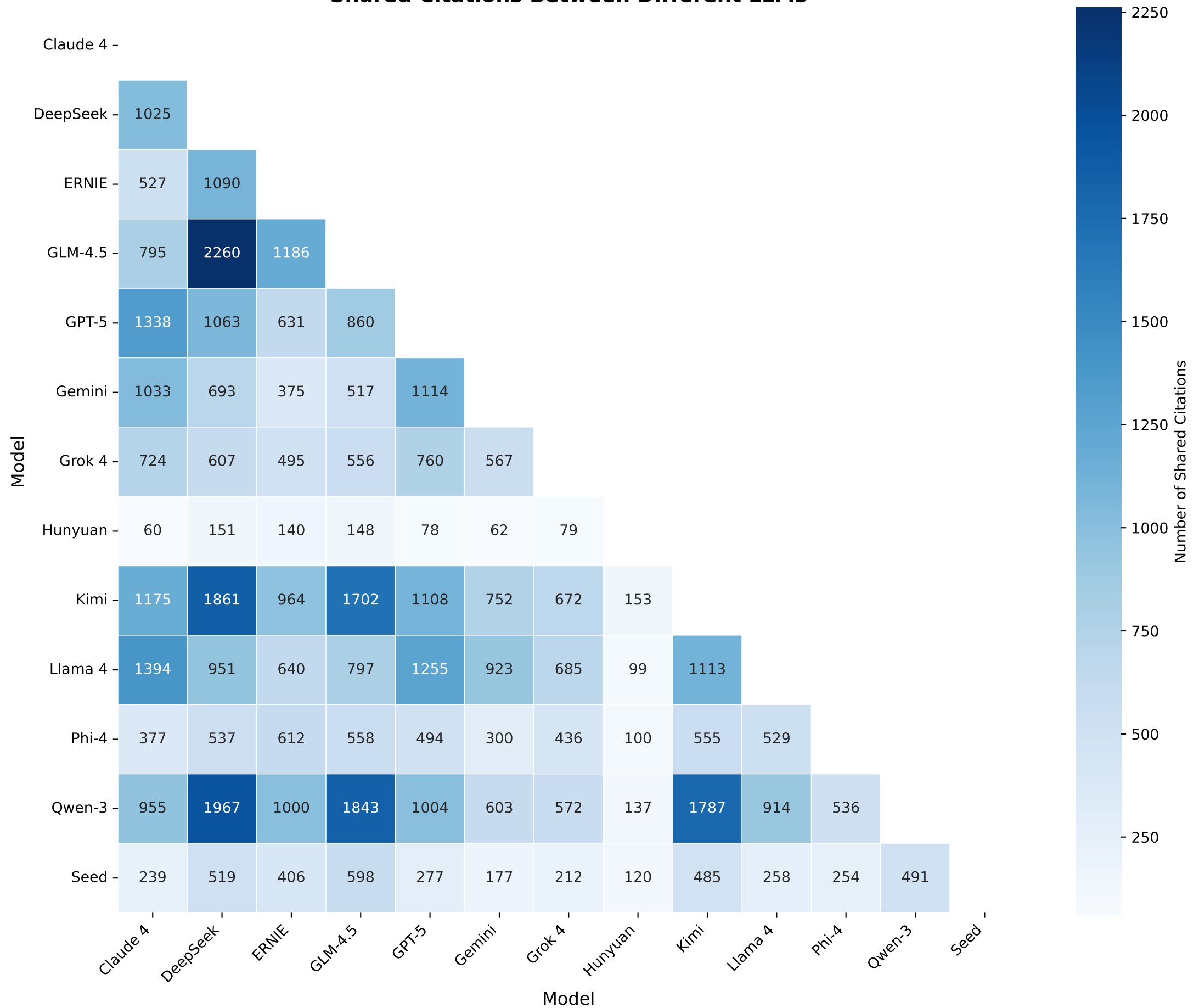
Cross-Model Citation Overlap (Lower Triangle) Shared Citations Between Different LLMs
