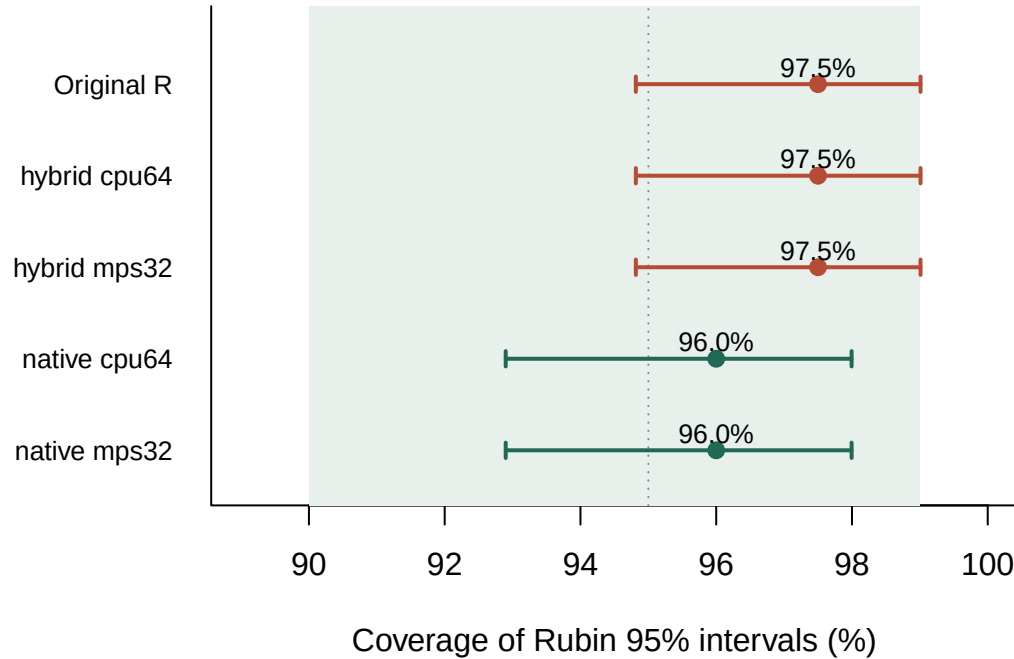
Absolute coverage Required interval inside [90%, 99%]
