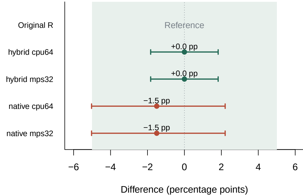
Paired difference from original R Required interval inside [-5, +5] pp
