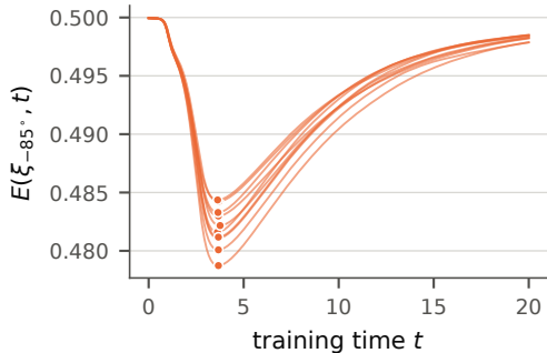
(c) ReLU at -85^\circ , 10 seed(s)
