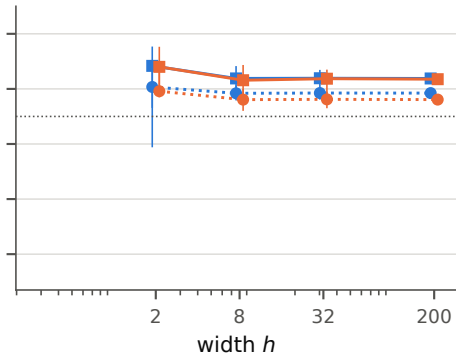
\mu = (1, 2), \sigma = 0.05 , pos init
