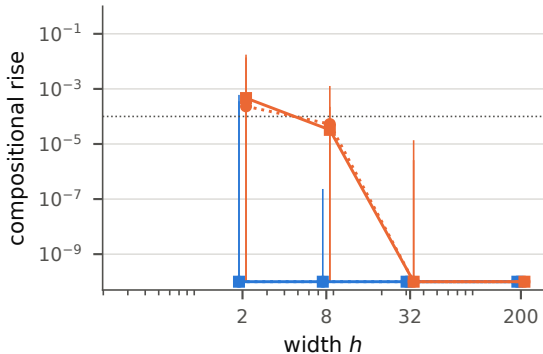
\mu = (1, 2), \sigma = 0.05 , iso init
