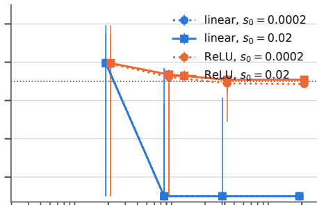
\mu = (1, 2), \sigma = 0.05 , pos init
