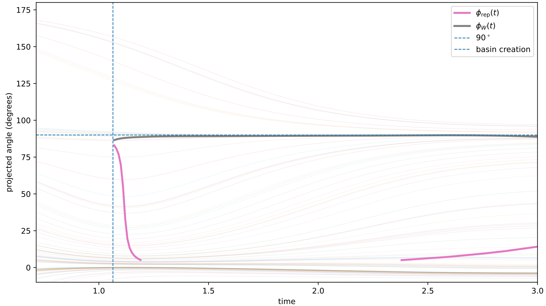
P0-B: O-transition trajectories vs. moving weak separatrix
