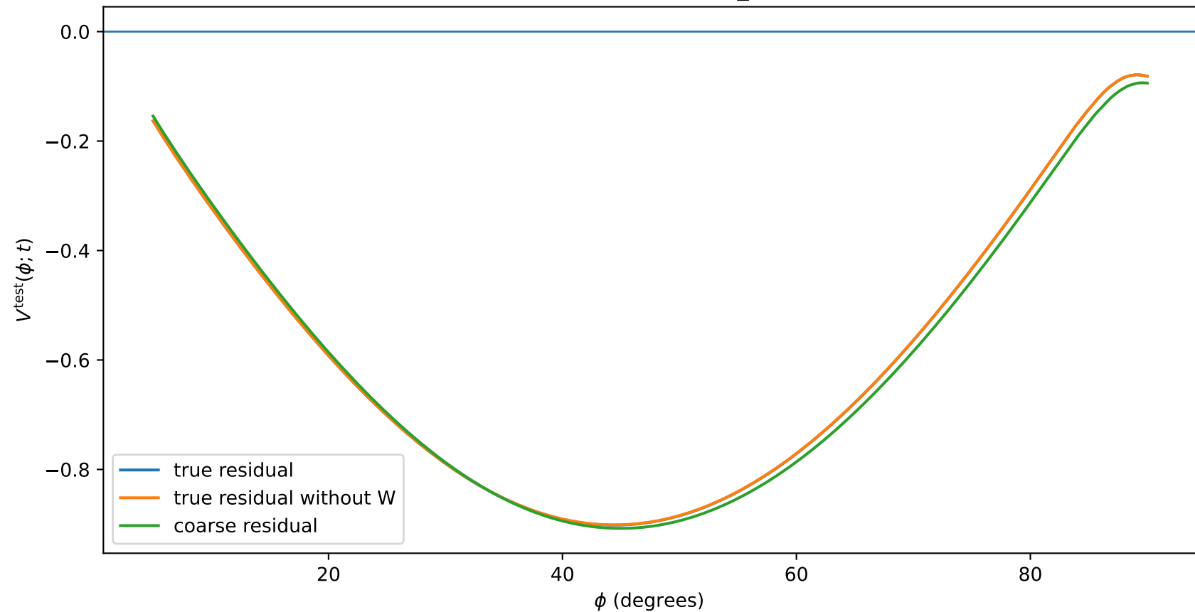
Weak test field: t=0.90 , m_{\text{eff}}=0.151
