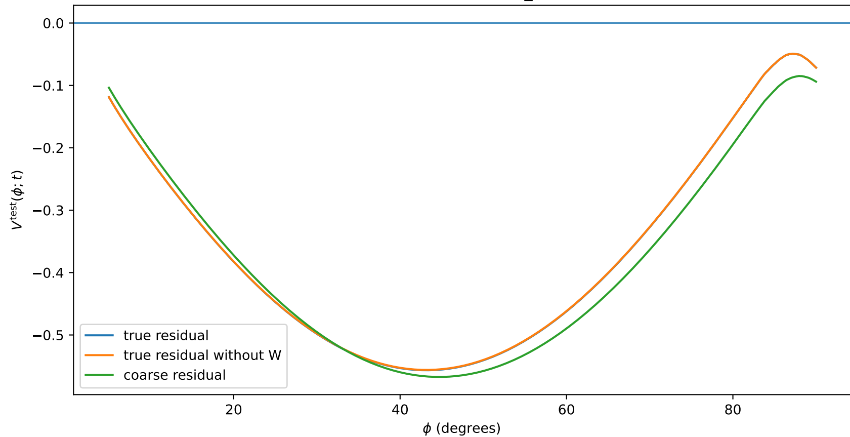
Weak test field: t=1.00 , m_{\text{eff}}=0.304
