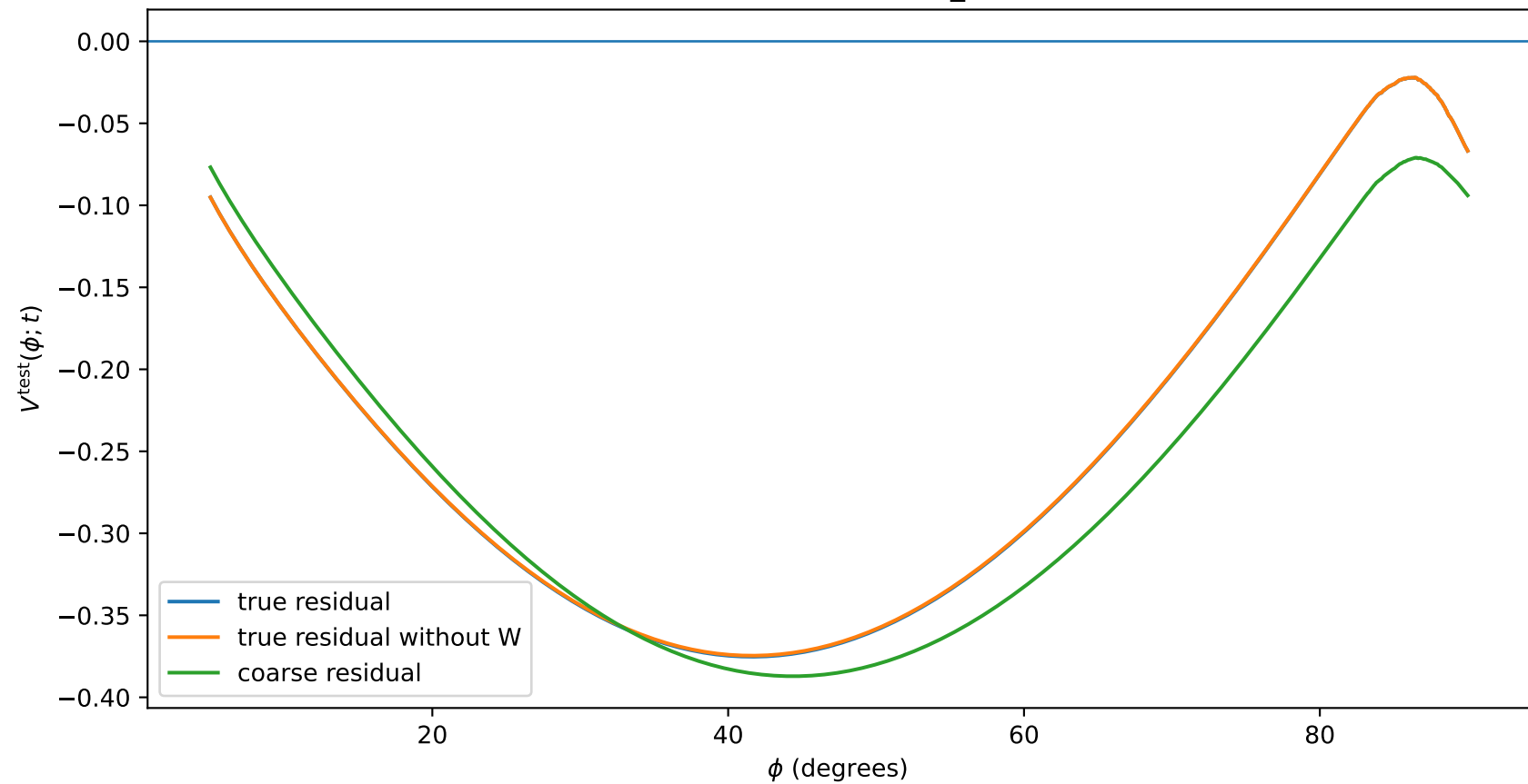
Weak test field: t=1.04 , m_{\text{eff}}=0.385
