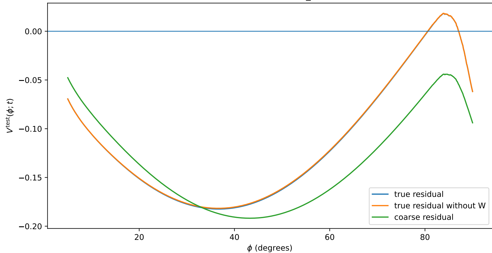
Weak test field: t=1.08 , m_{\text{eff}}=0.473
