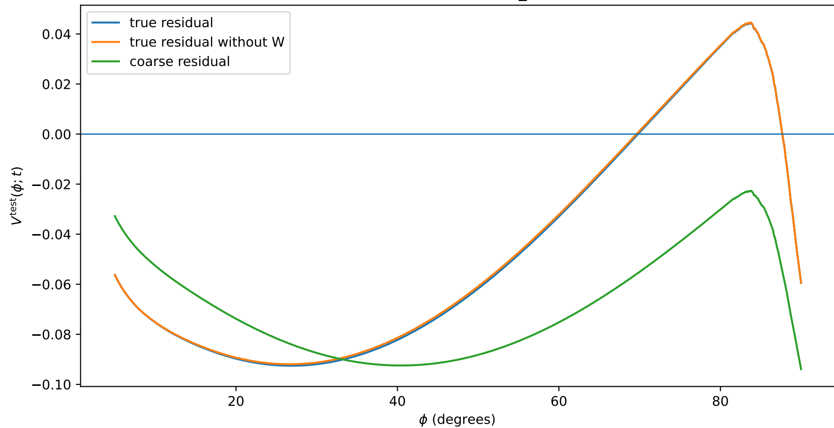
Weak test field: t=1.10 , m_{\text{eff}}=0.518
