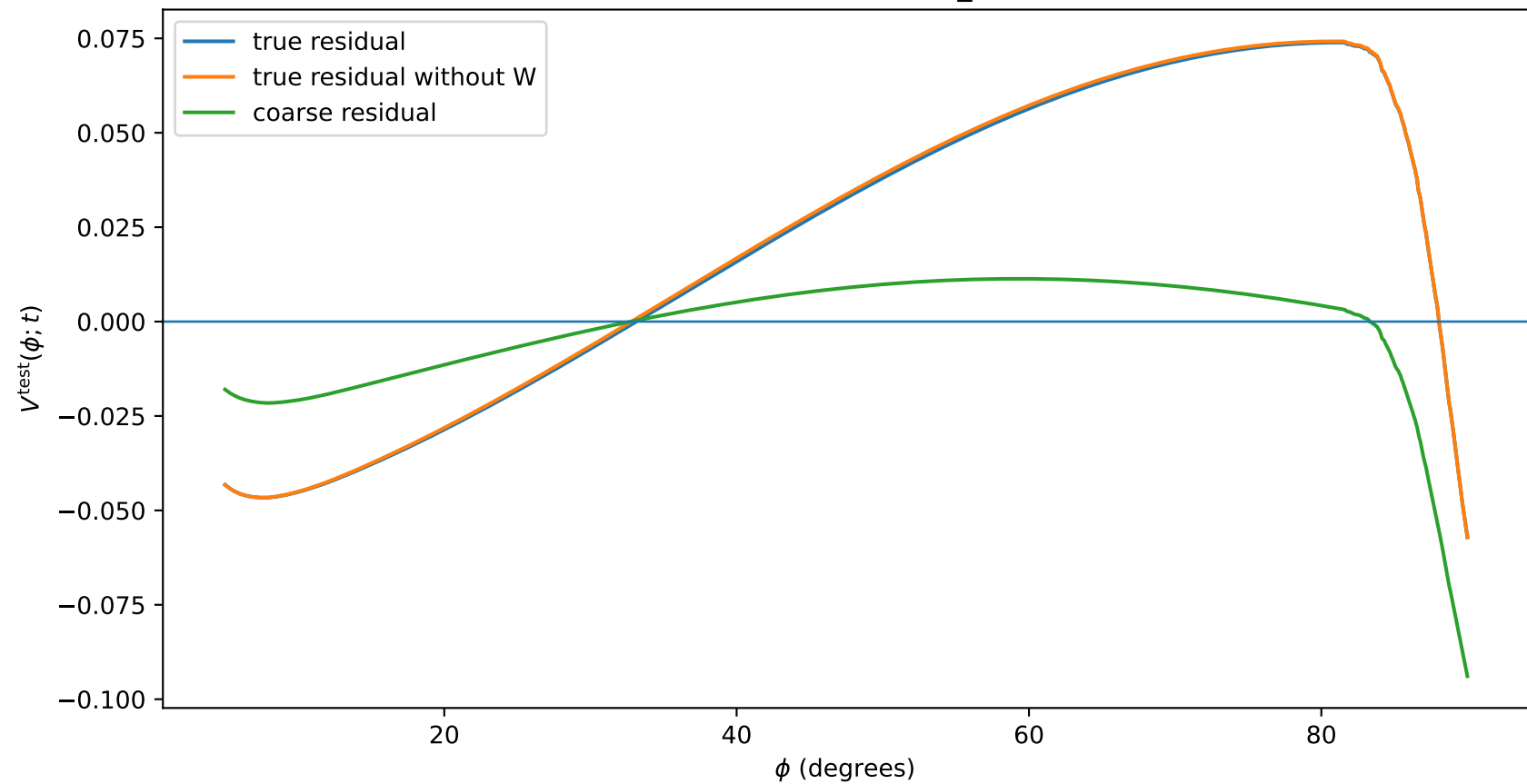
Weak test field: t=1.12 , m_{\text{eff}}=0.563
