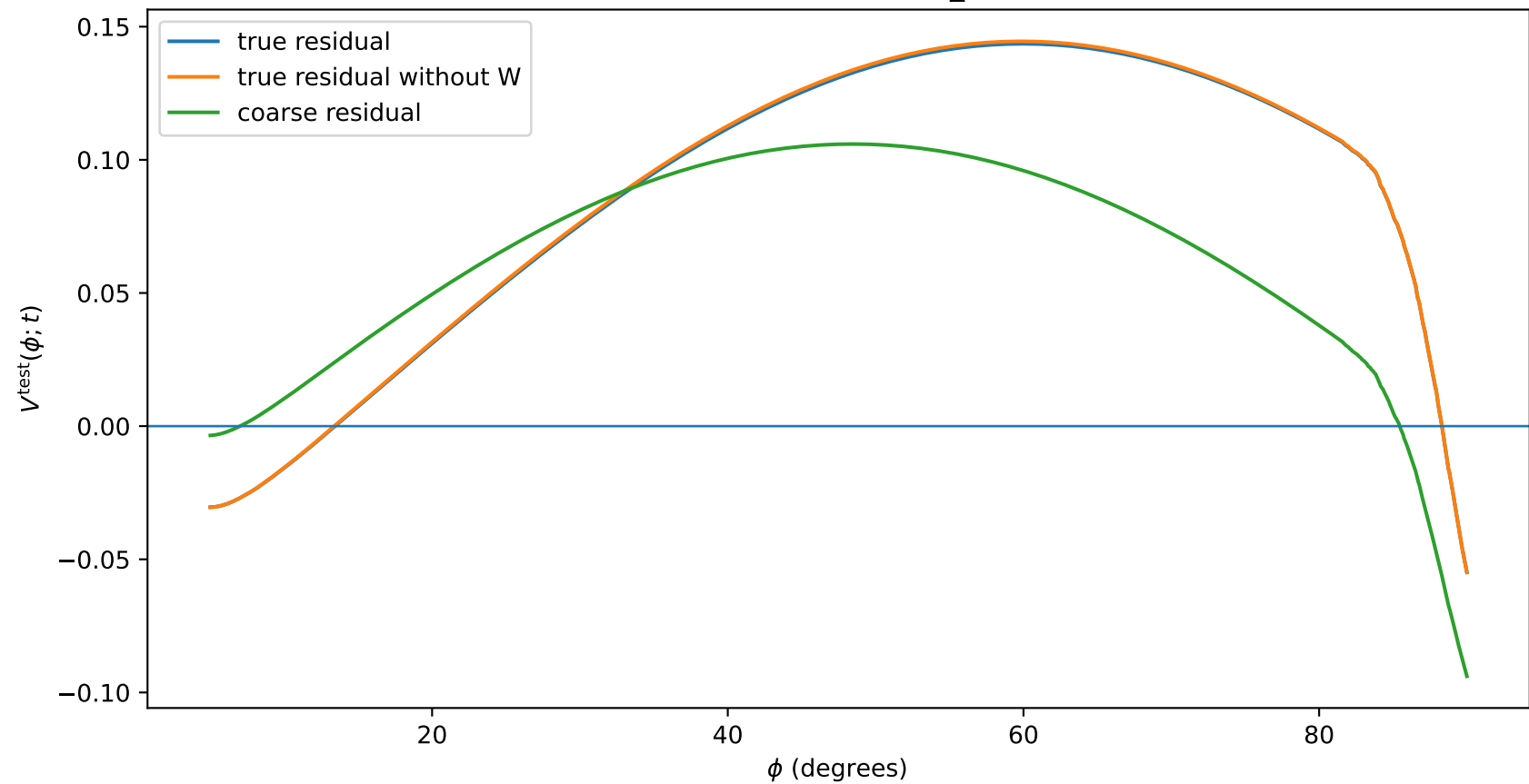
Weak test field: t=1.14 , m_{\text{eff}}=0.606
