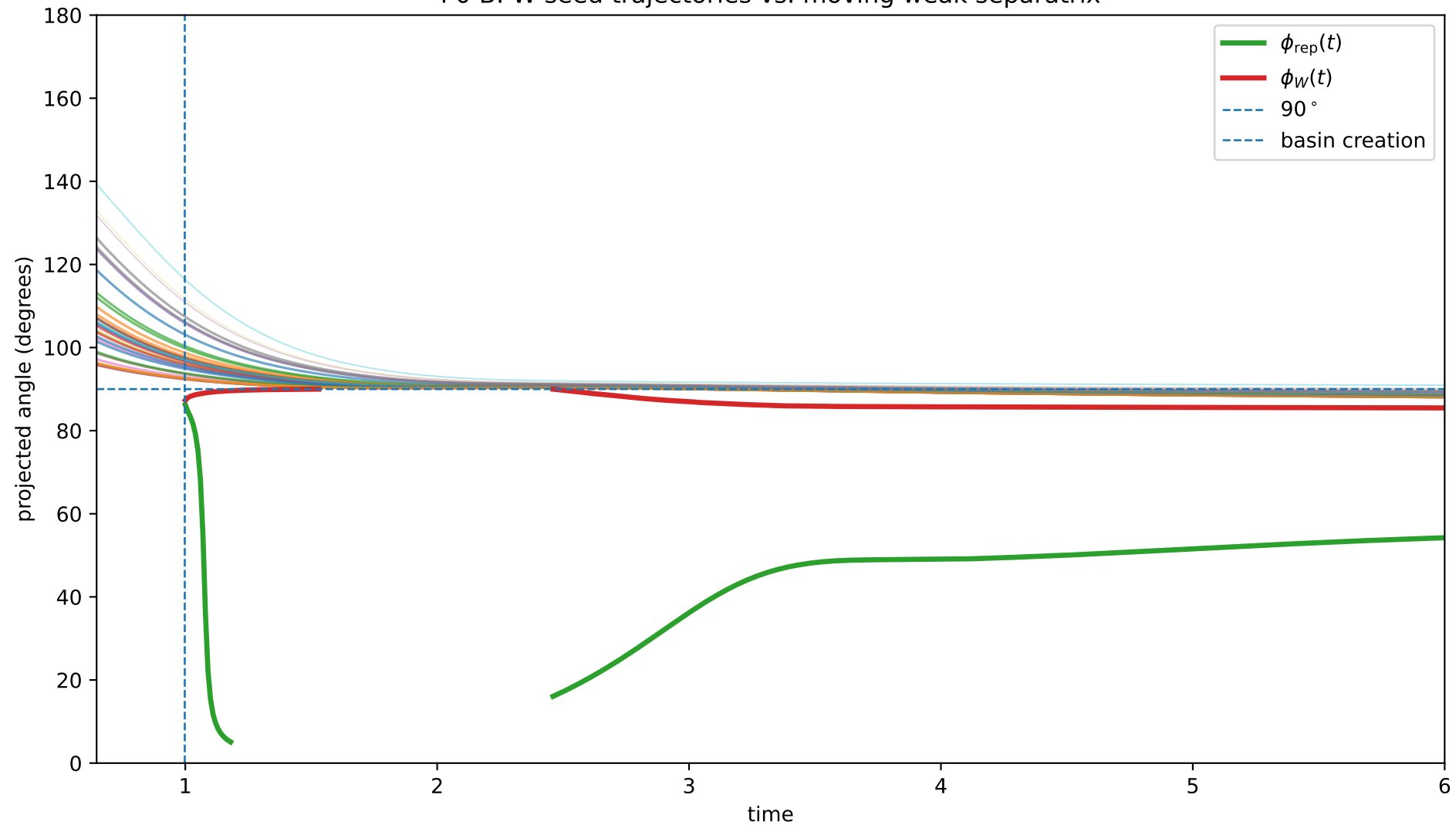
P0-B: W-seed trajectories vs. moving weak separatrix
