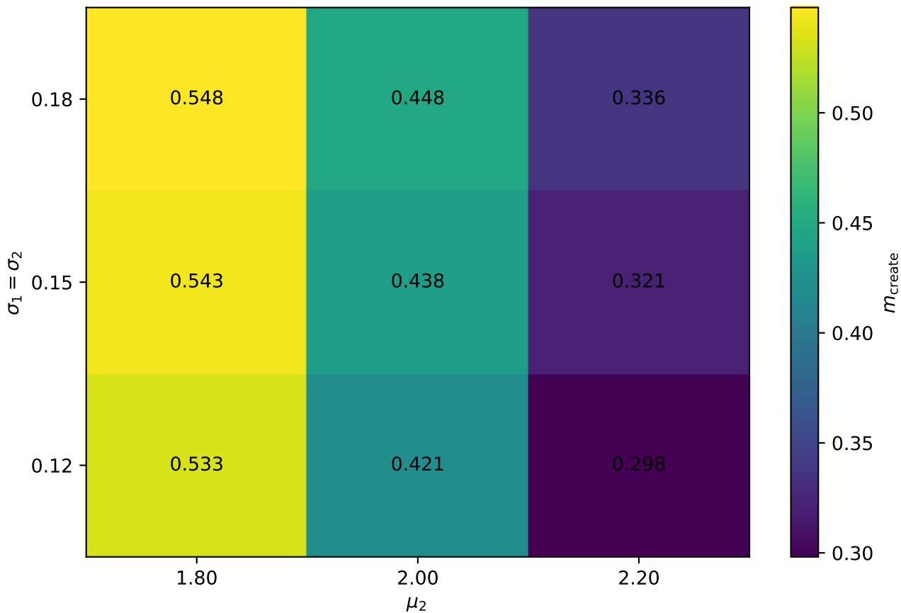
P0-D: true weak-basin creation threshold
