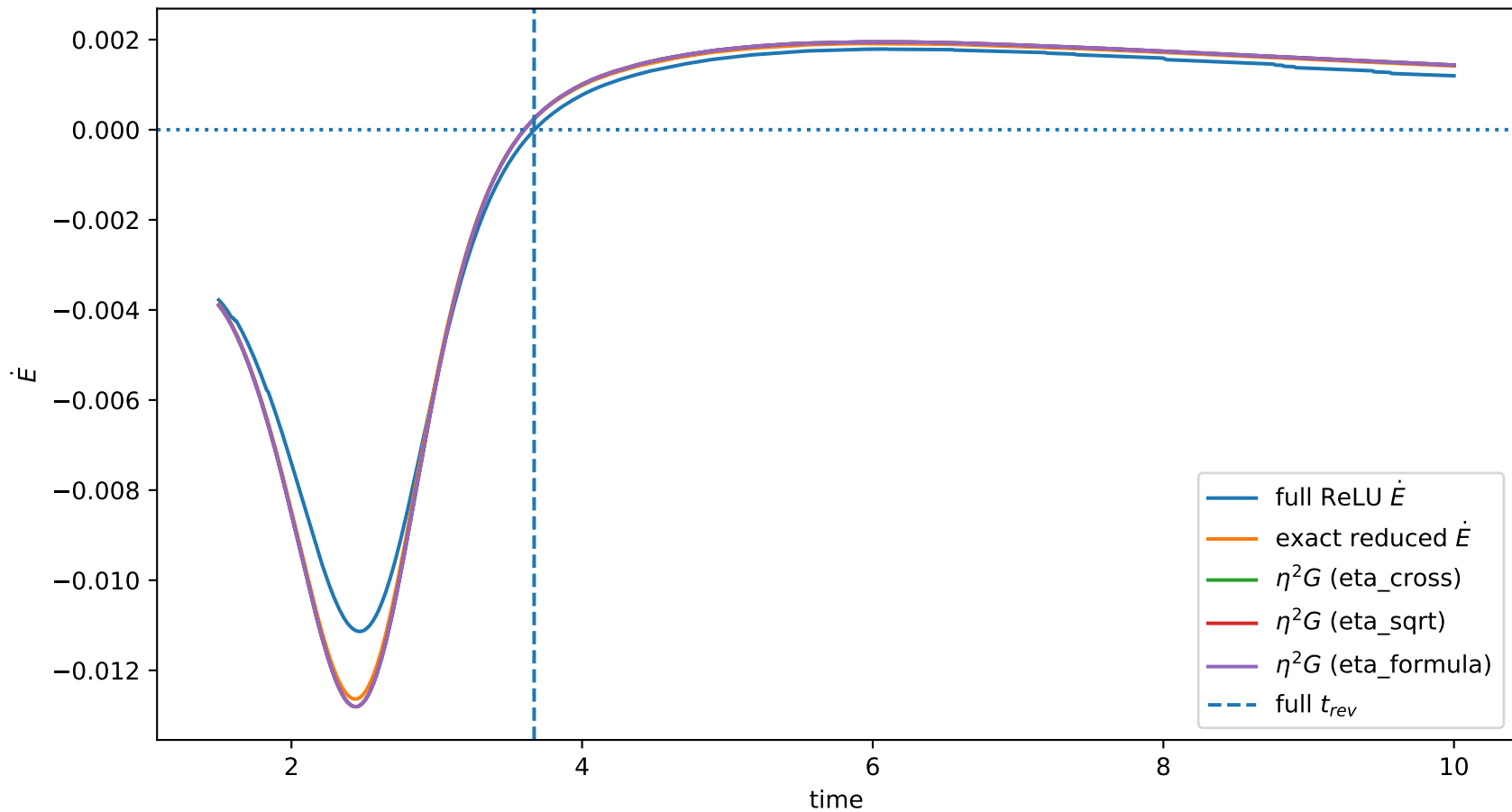
Canonical near-boundary normal-form check: \psi = -85^\circ
