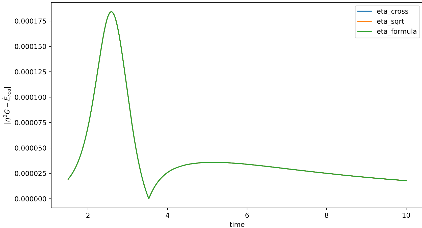
Normal-form derivative approximation error
