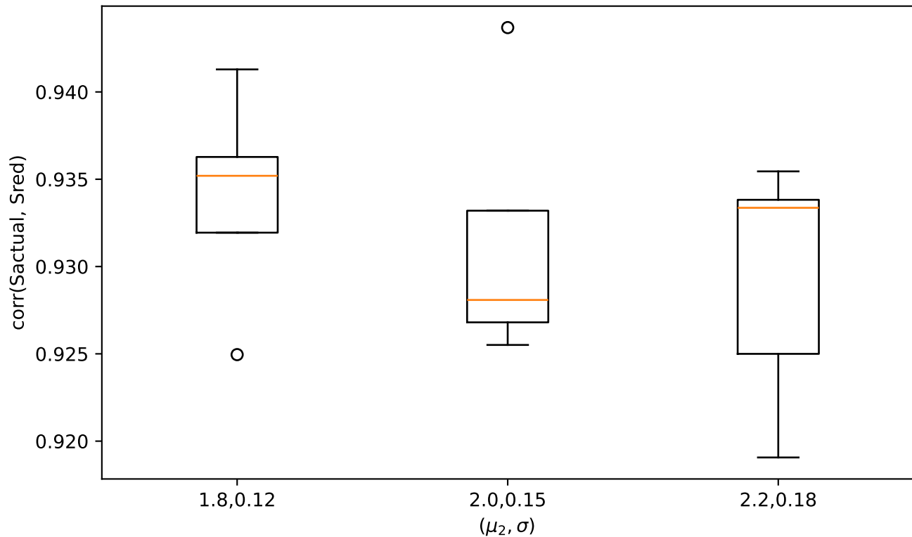
Multi-seed robustness
