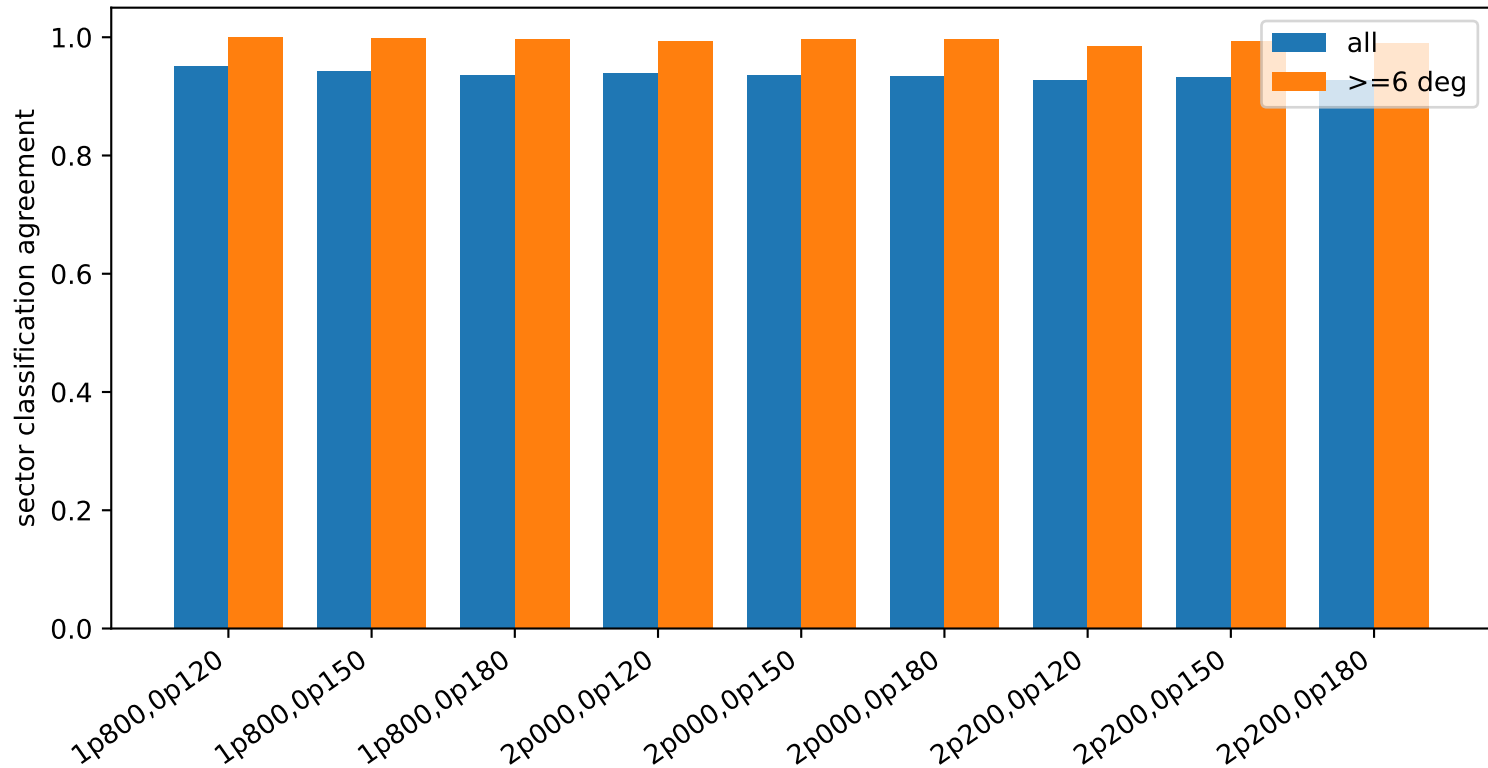
Full vs reduced OOD sector classification
