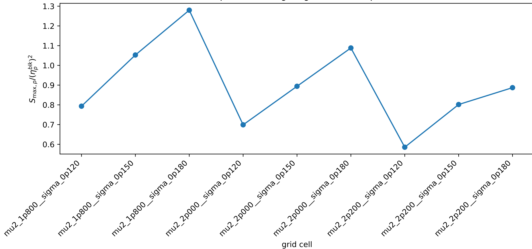
Amplitude scaling diagnostic, block p=1
