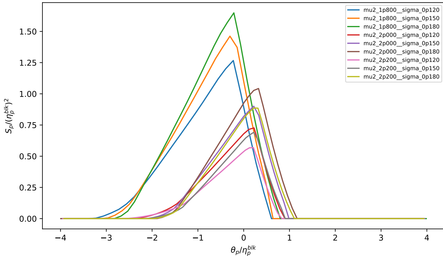
Preregistered near-boundary profile collapse, p=2
