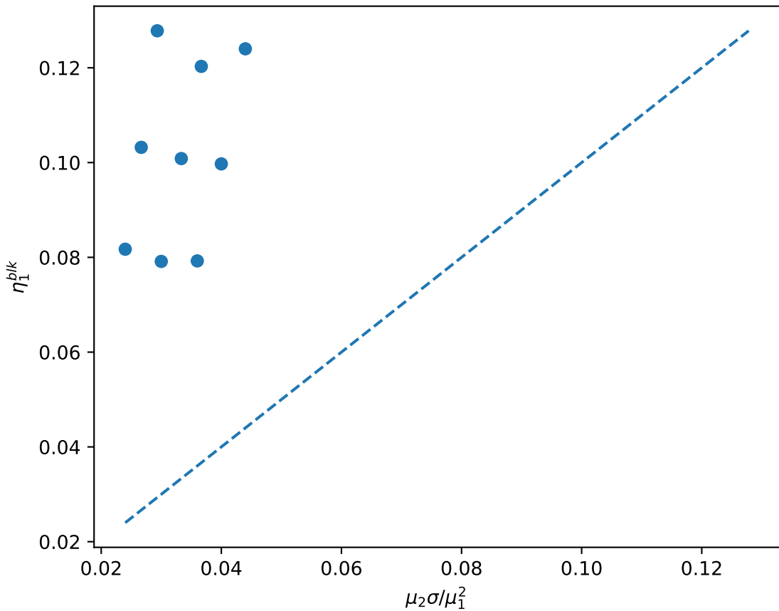
Strong block: max leakage scale vs parameter formula
