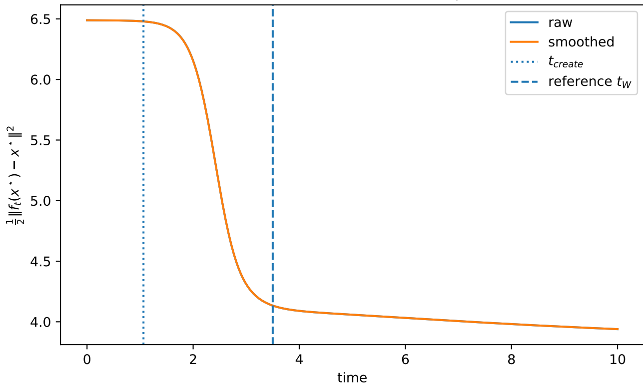
Check B: ReLU OOD loss (mp)
