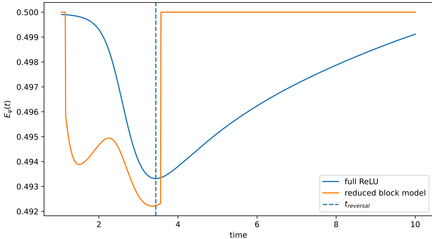
OOD loss decomposition: \psi = 176.0^\circ
