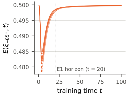
(a) ReLU at -85^\circ , 10 seeds
