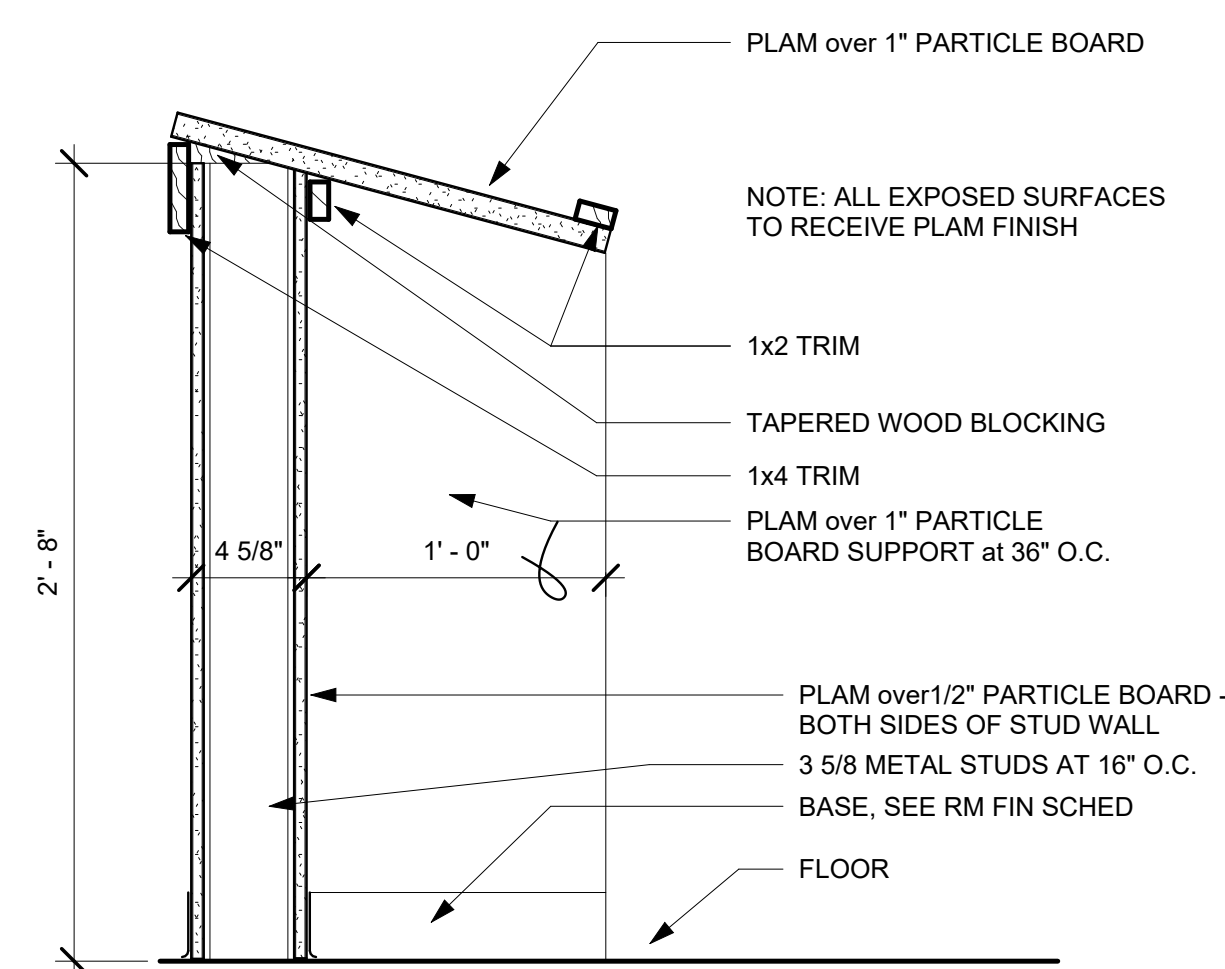
③ Fixed Student Desk 1 1/2" = 1'-0"
