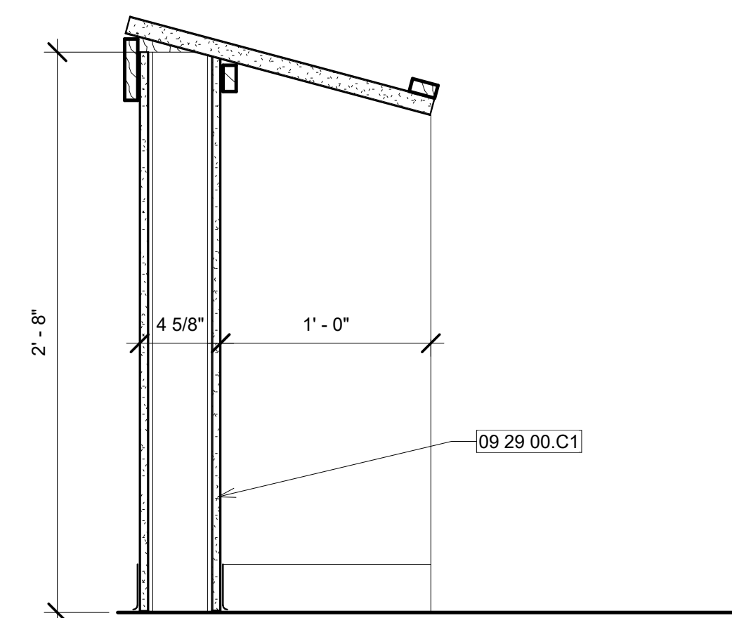
7 Fixed Student Desk - KEYNOTES 1 1/2" = 1'-0"
