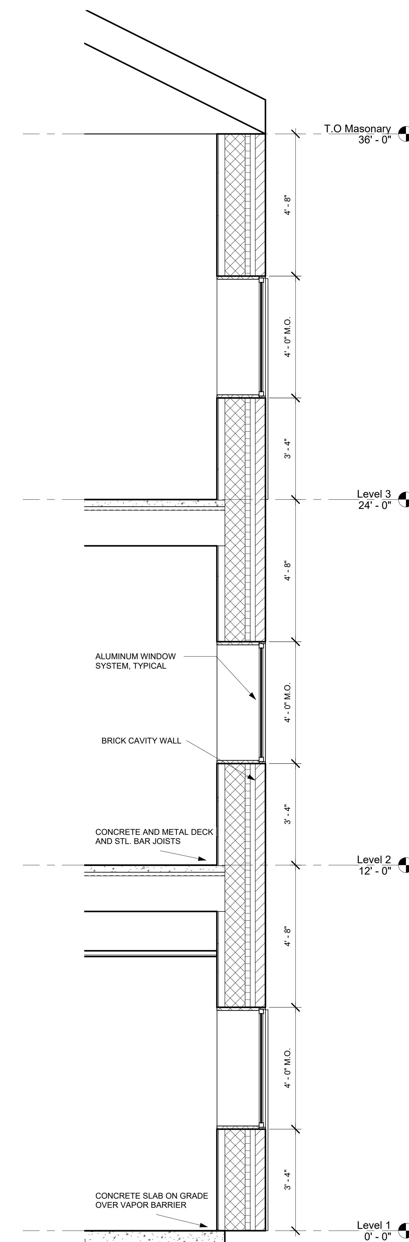
③ Cross Section 1 - Callout 1 1/2" = 1'-0"
