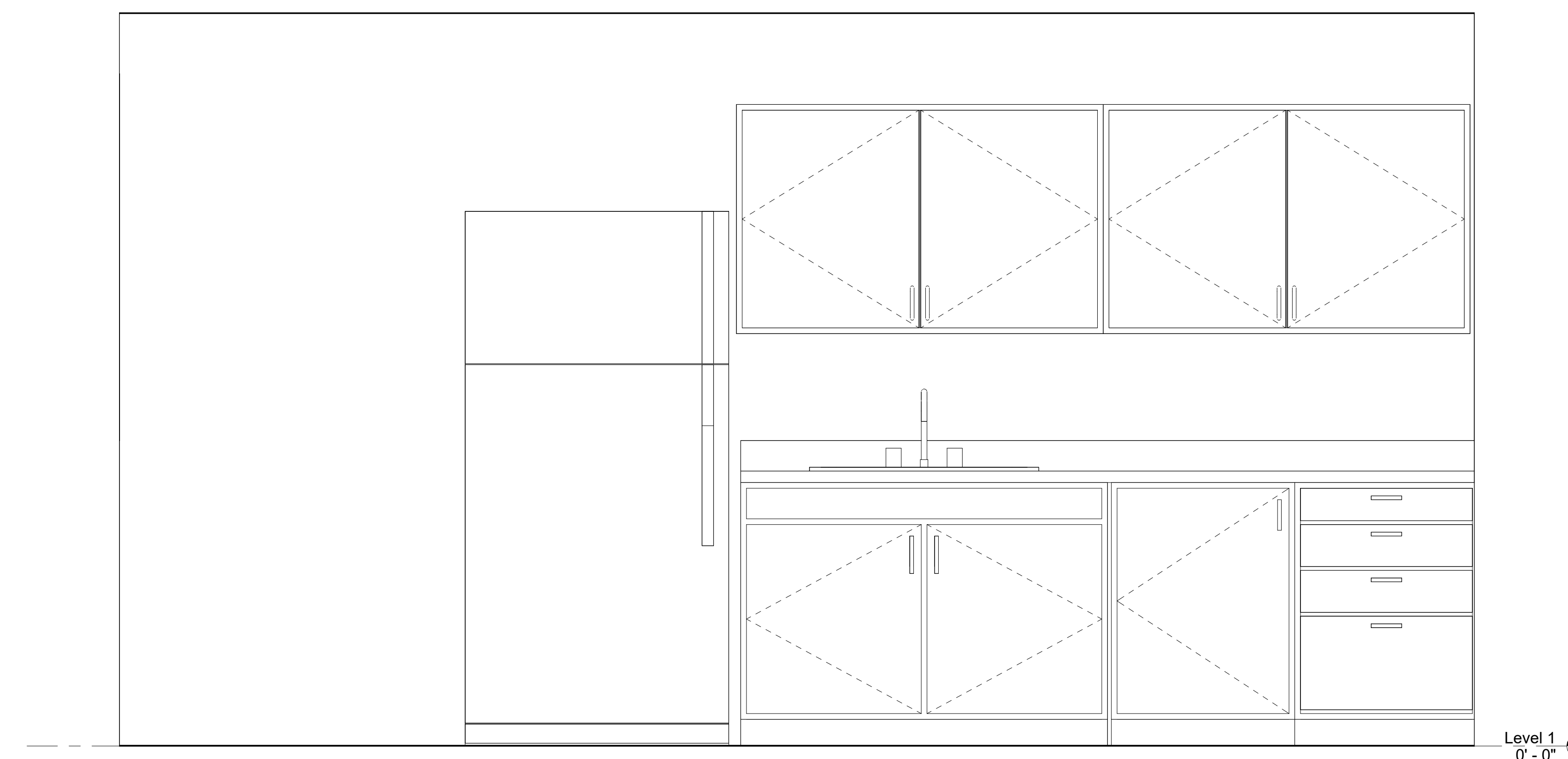
① Break Room East 1" = 1'-0"
