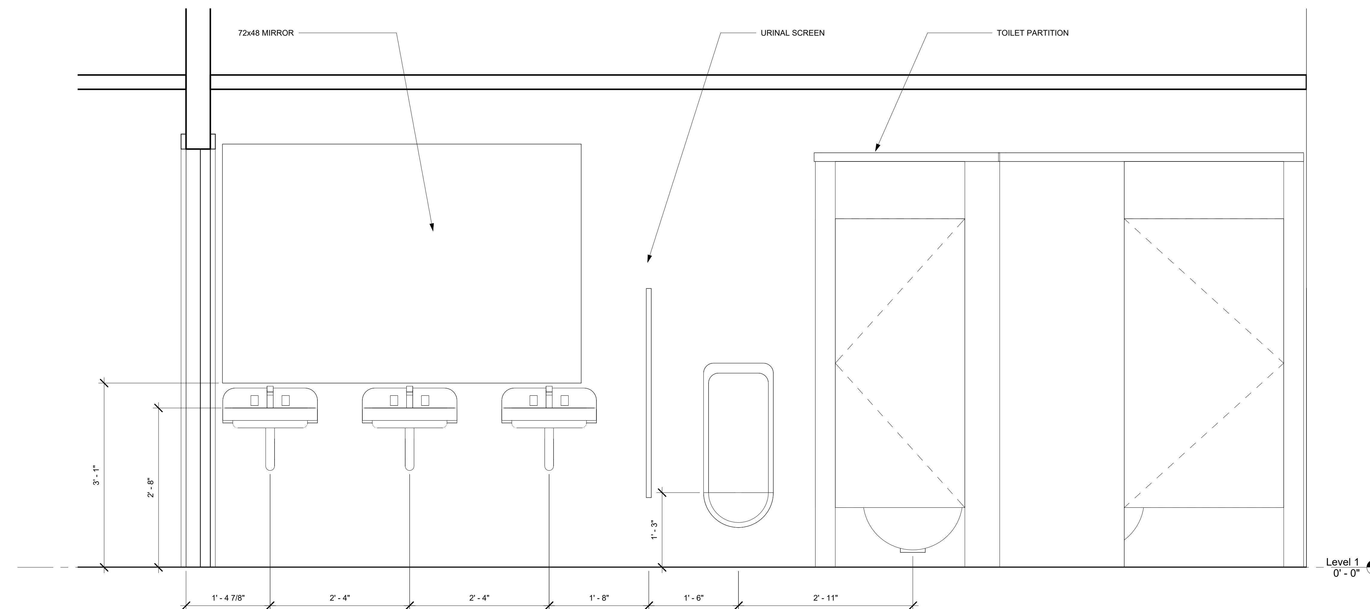
2 Mens Restroom 1" = 1'-0"
