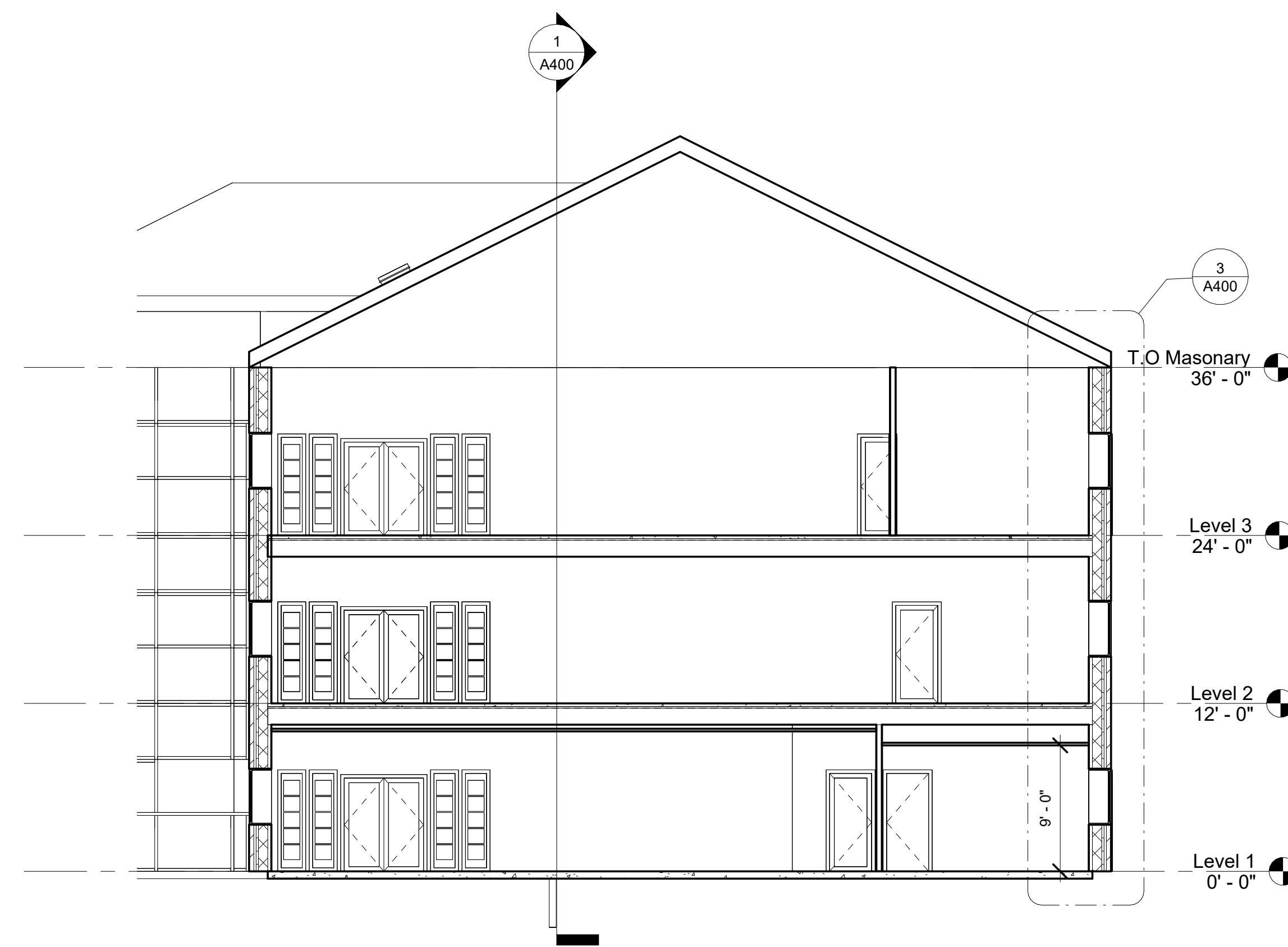
② Cross Section 1 1/8" = 1'-0"
