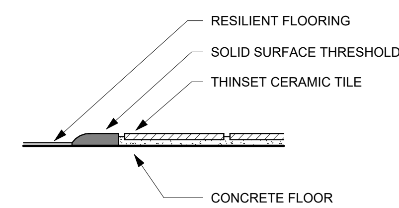
8 Floor Transition Detail 3" = 1'-0"
