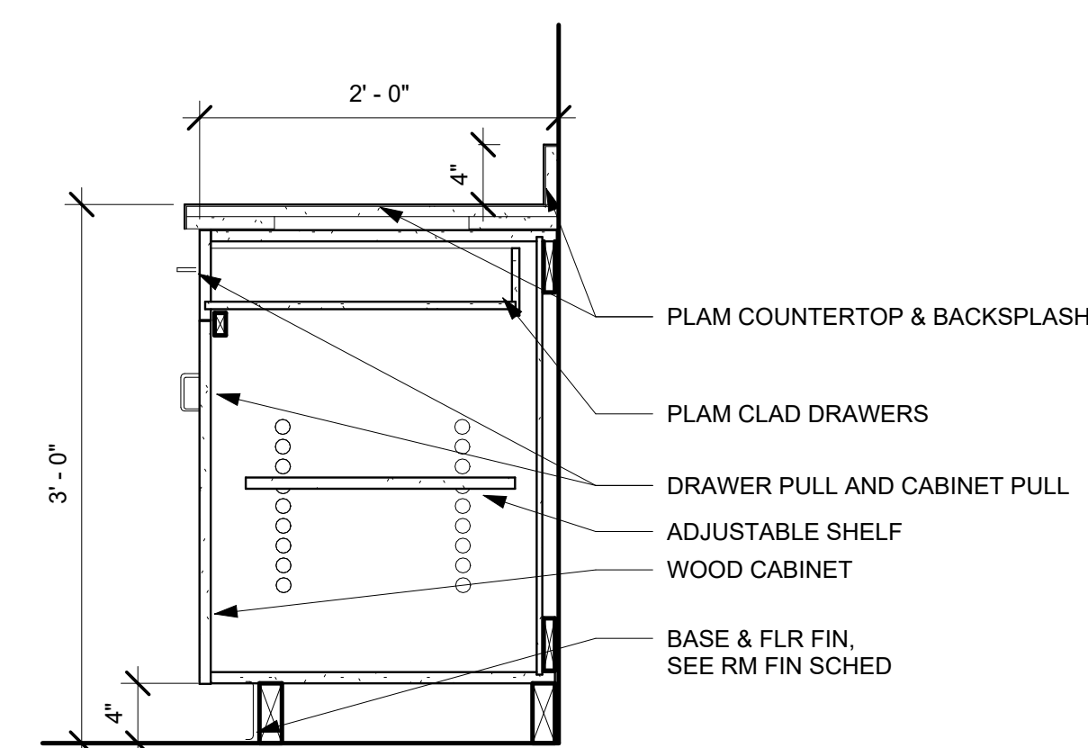
1 Base Cabinet Detail 1" = 1'-0"
