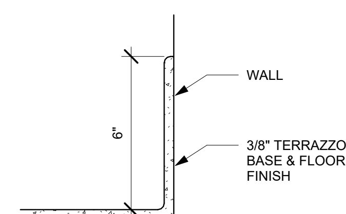
6 Terrazzo Base Detail 3" = 1'-0"
