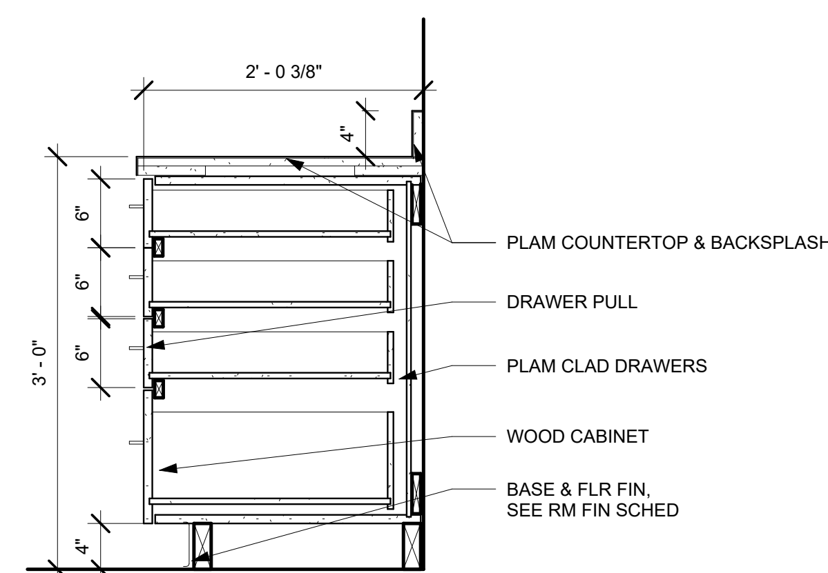
② Base Cabinet Detail - Drawers 1" = 1'-0"
