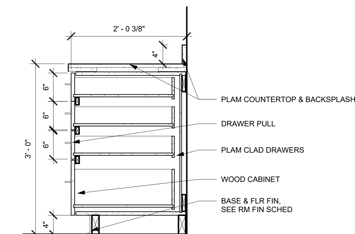
② Base Cabinet Detail - Drawers 1" = 1'-0"
