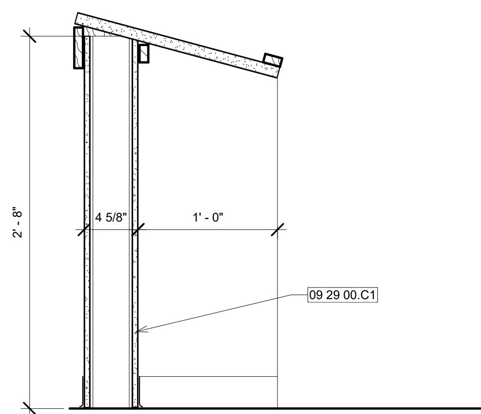
7 Fixed Student Desk - KEYNOTES 1 1/2" = 1'-0"
