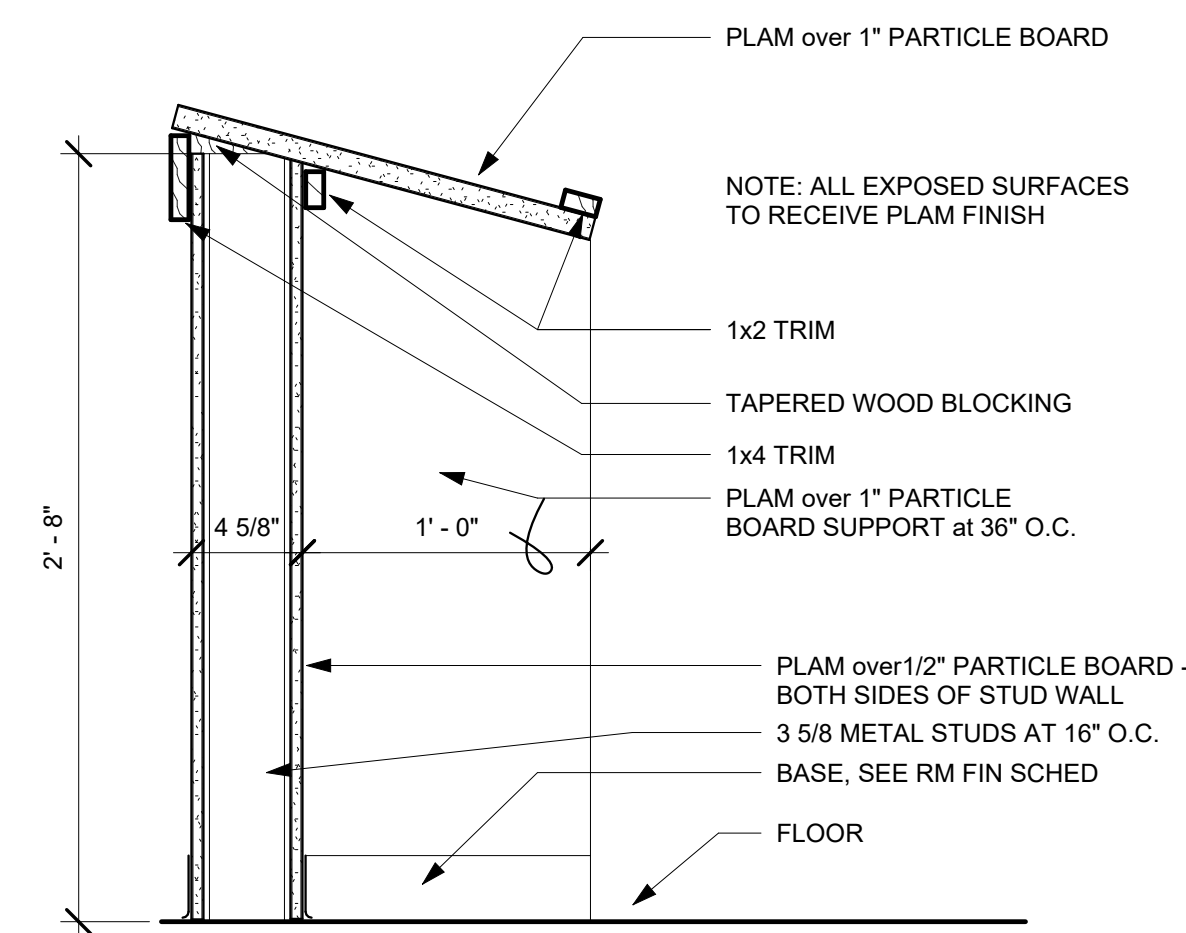
③ Fixed Student Desk 1 1/2" = 1'-0"
