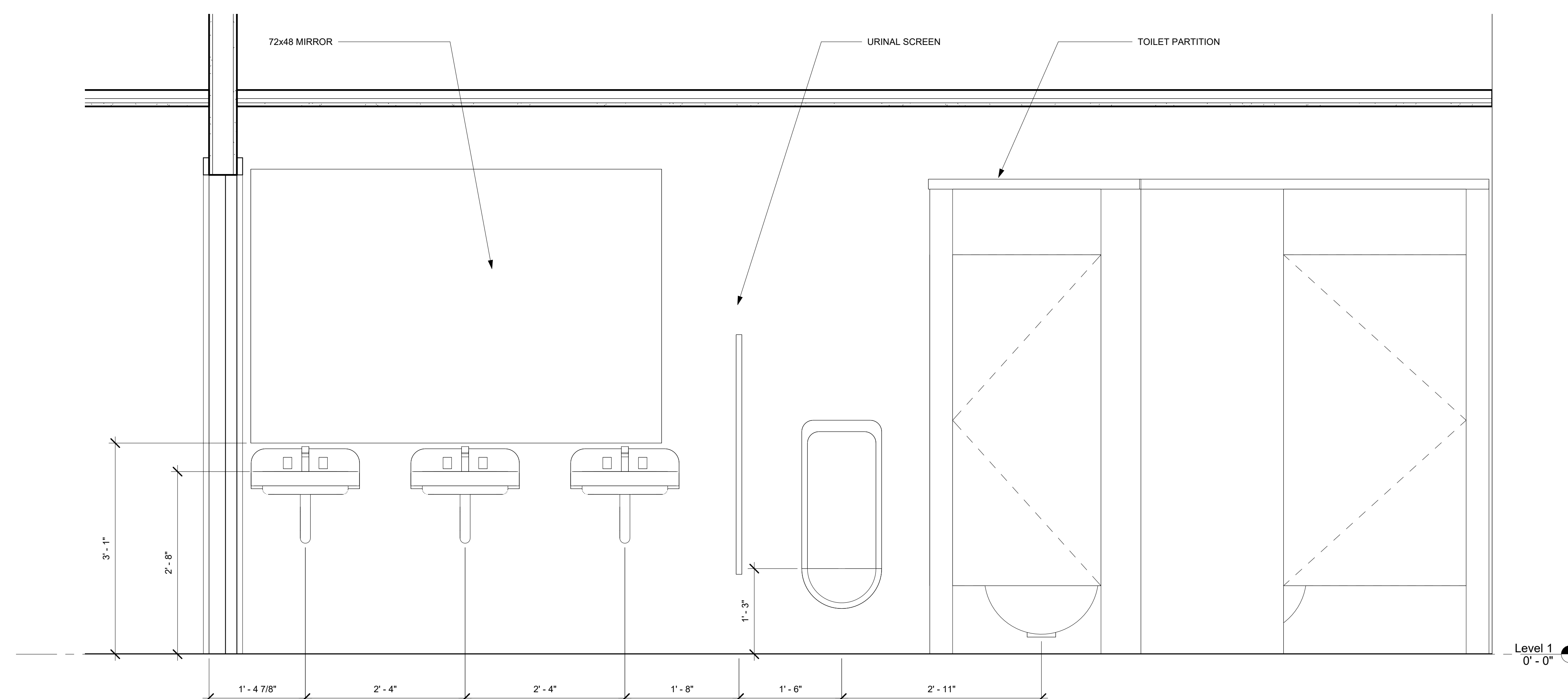
② Mens Restroom 1" = 1'-0"
