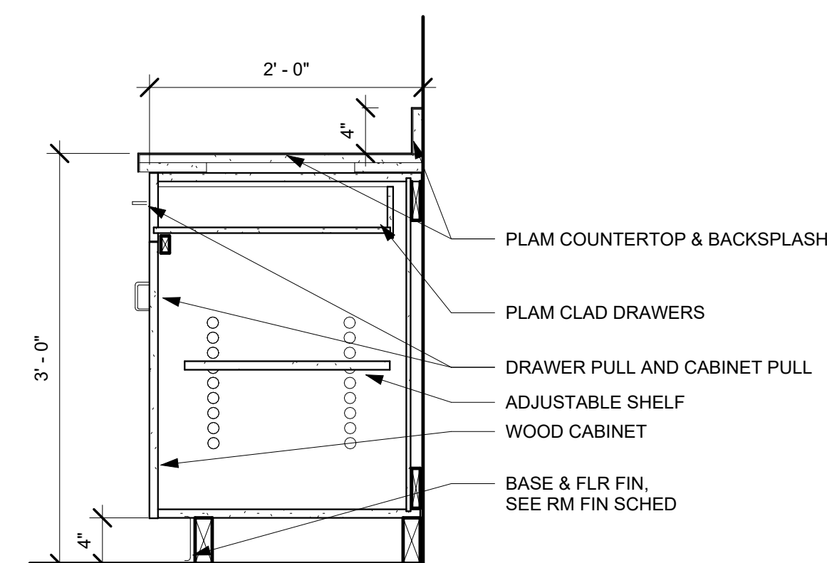
1 Base Cabinet Detail 1" = 1'-0"
