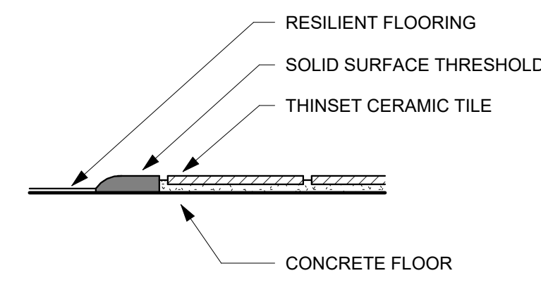
8 Floor Transition Detail 3" = 1'-0"
