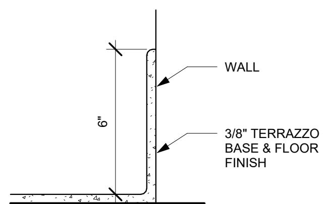
6 Terrazzo Base Detail 3" = 1'-0"
