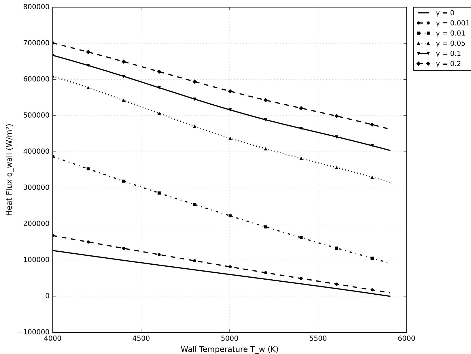
Abacus: q_{\text{wall}}(\gamma, T_w)
