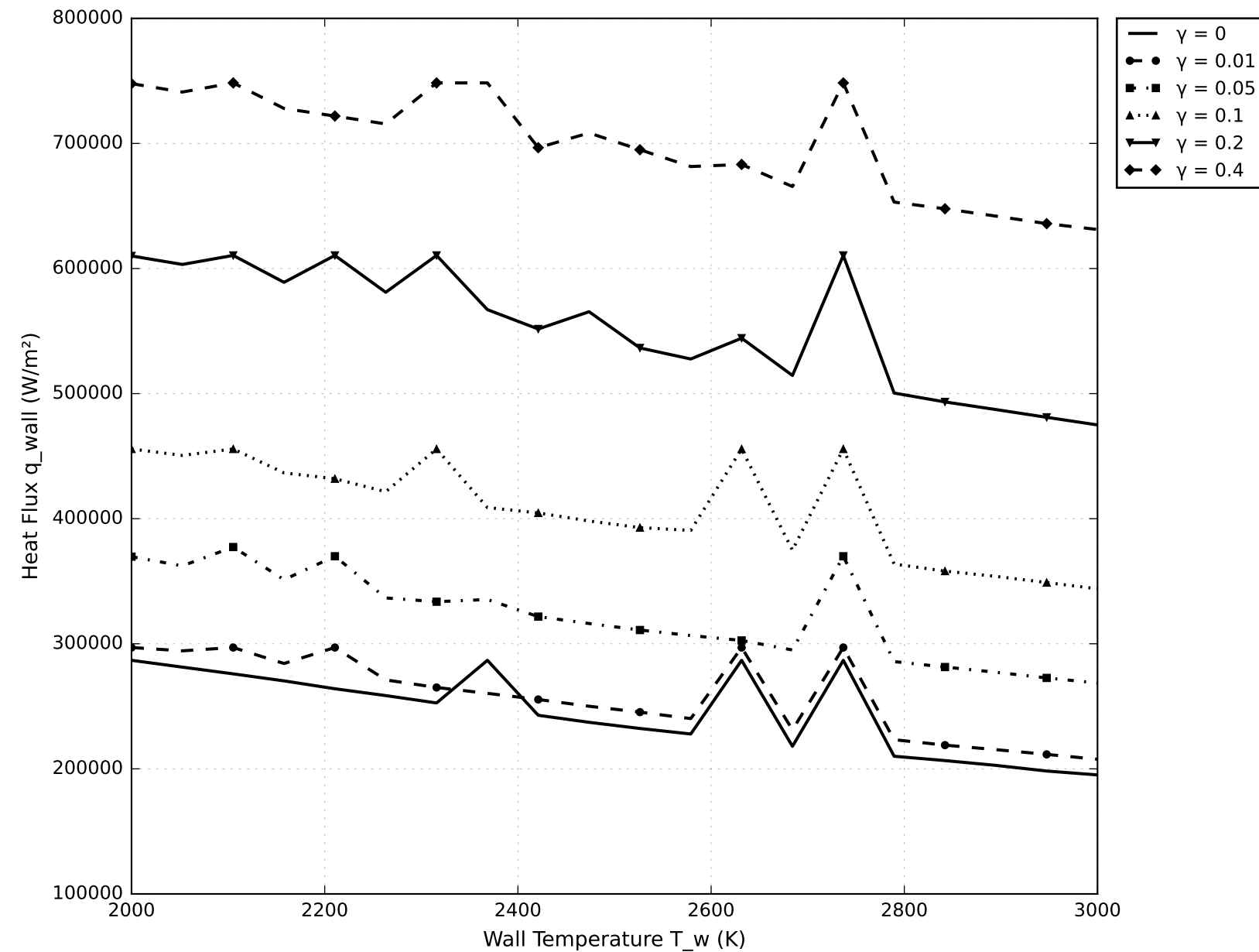
Abaque: q_{\text{wall}}(\gamma, T_w)
