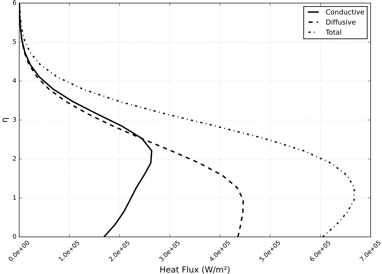
Station 000 - Dimensional Heat Flux Profiles
