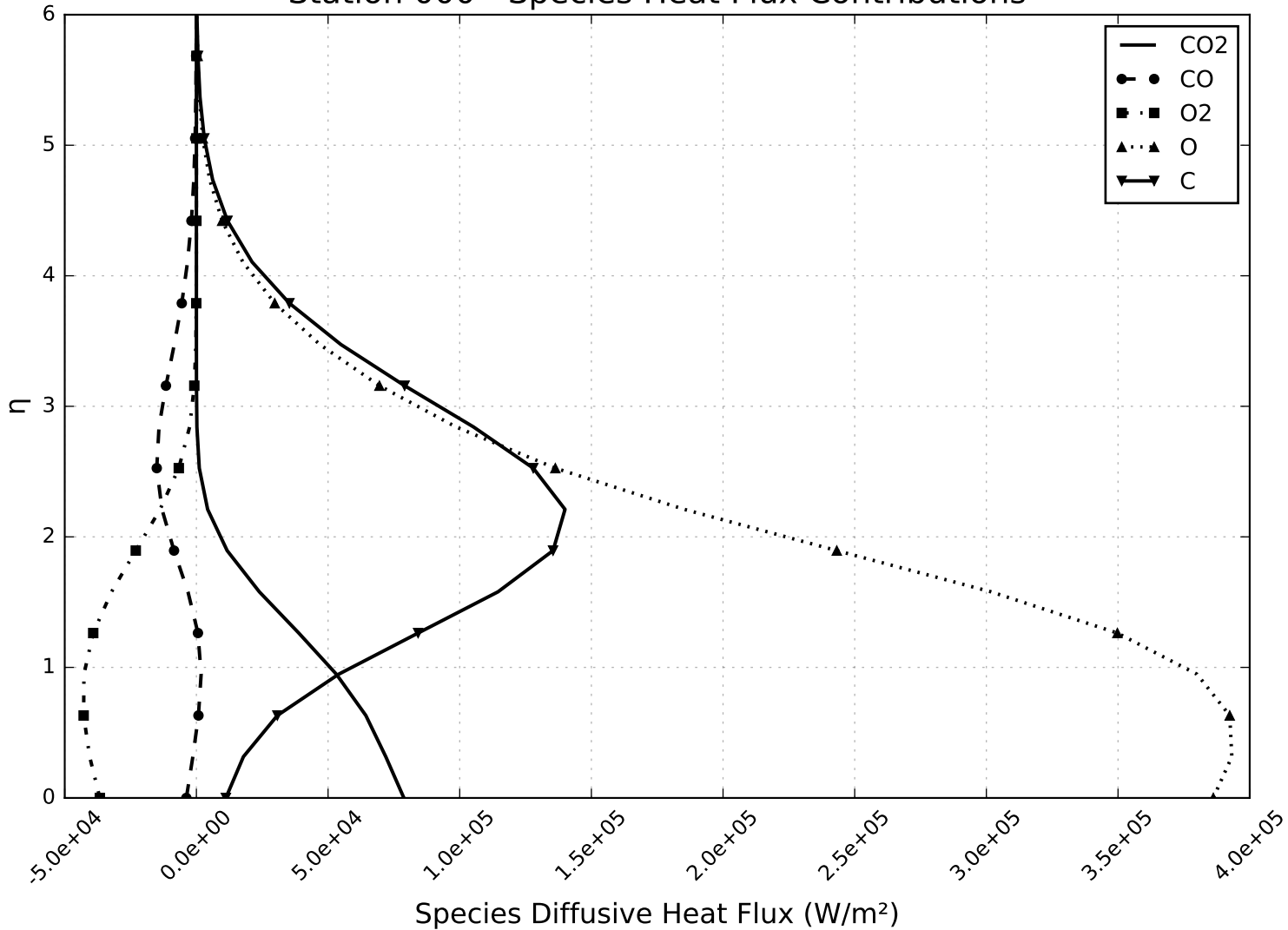
Station 000 - Species Heat Flux Contributions
