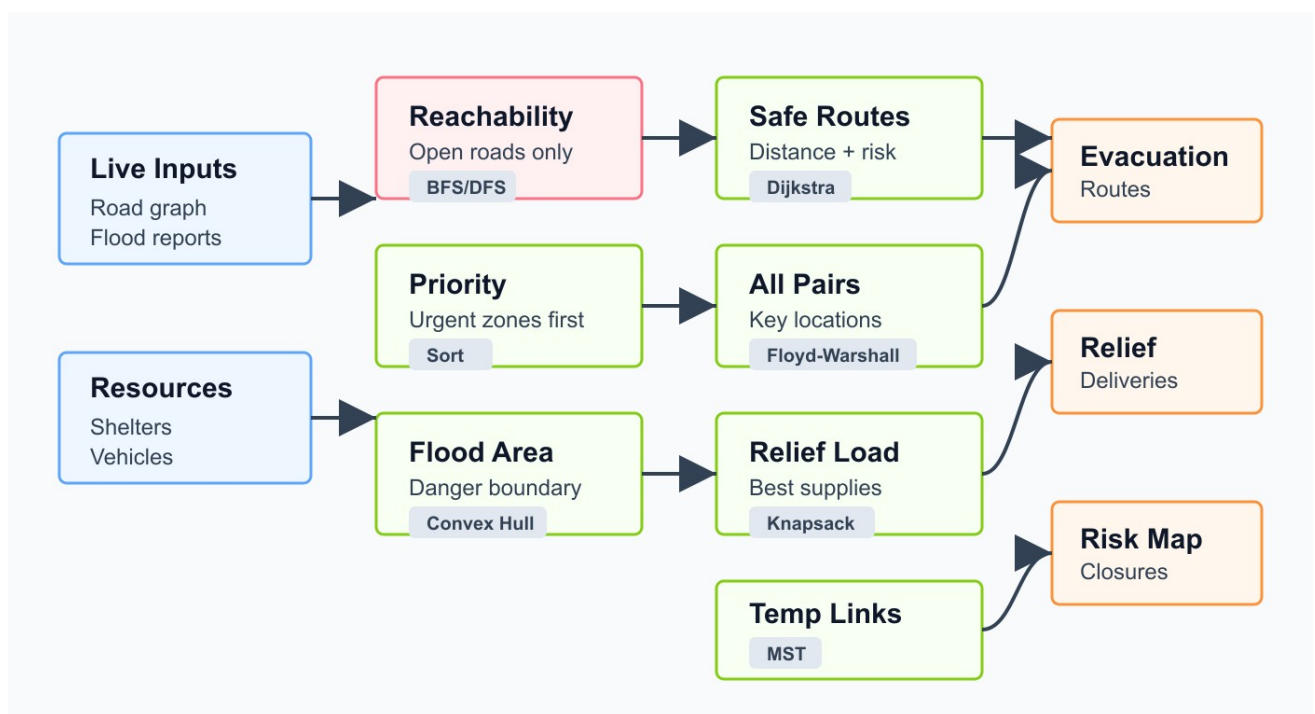
Figure 1: proposed pipeline connecting the real world flood-related problems to algorithms
