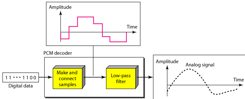
Figure: Components of PCM decoder
