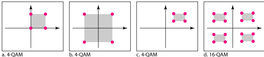
Figure: QAM constellation example
