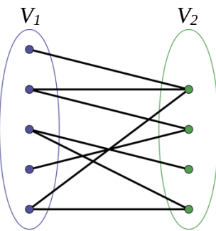
Example of a bipartite graph
