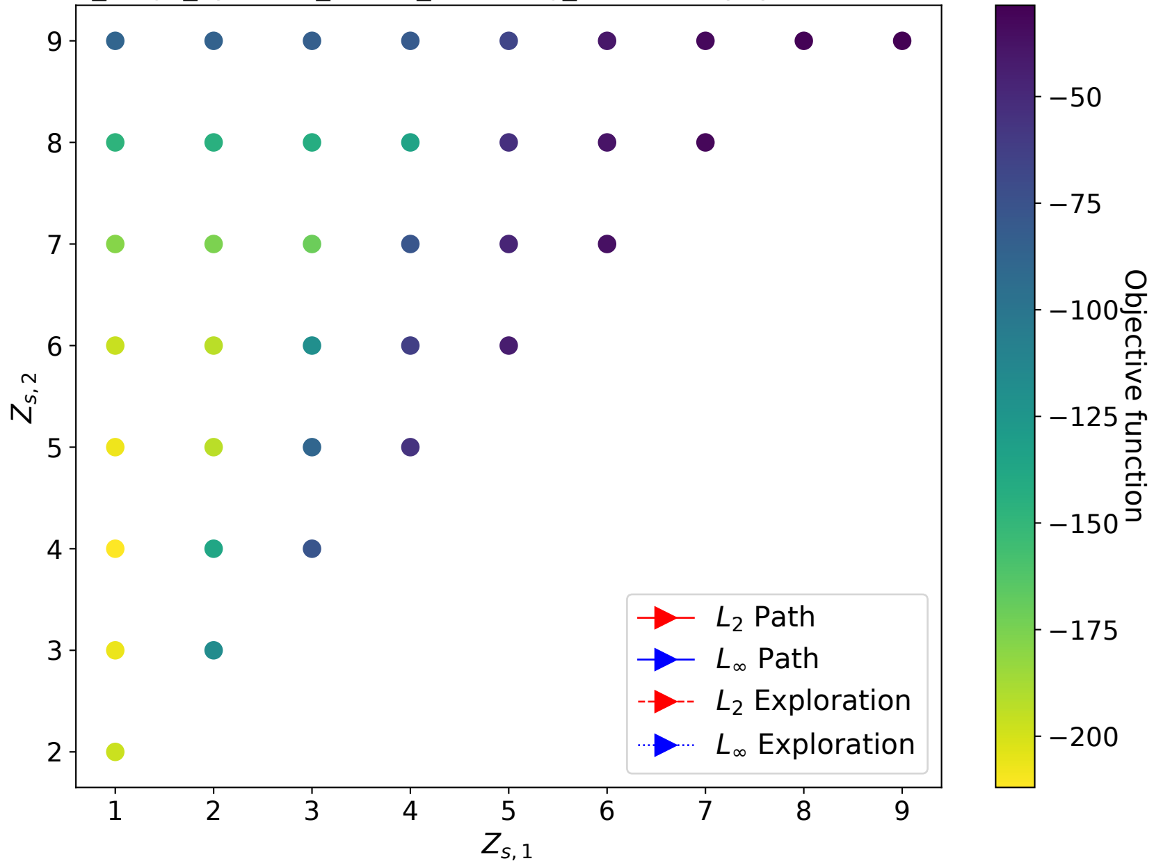
LDBD nine_stage_dynamic_model_switching_nonlinear ipopt Transfer (L2 vs Linf)
