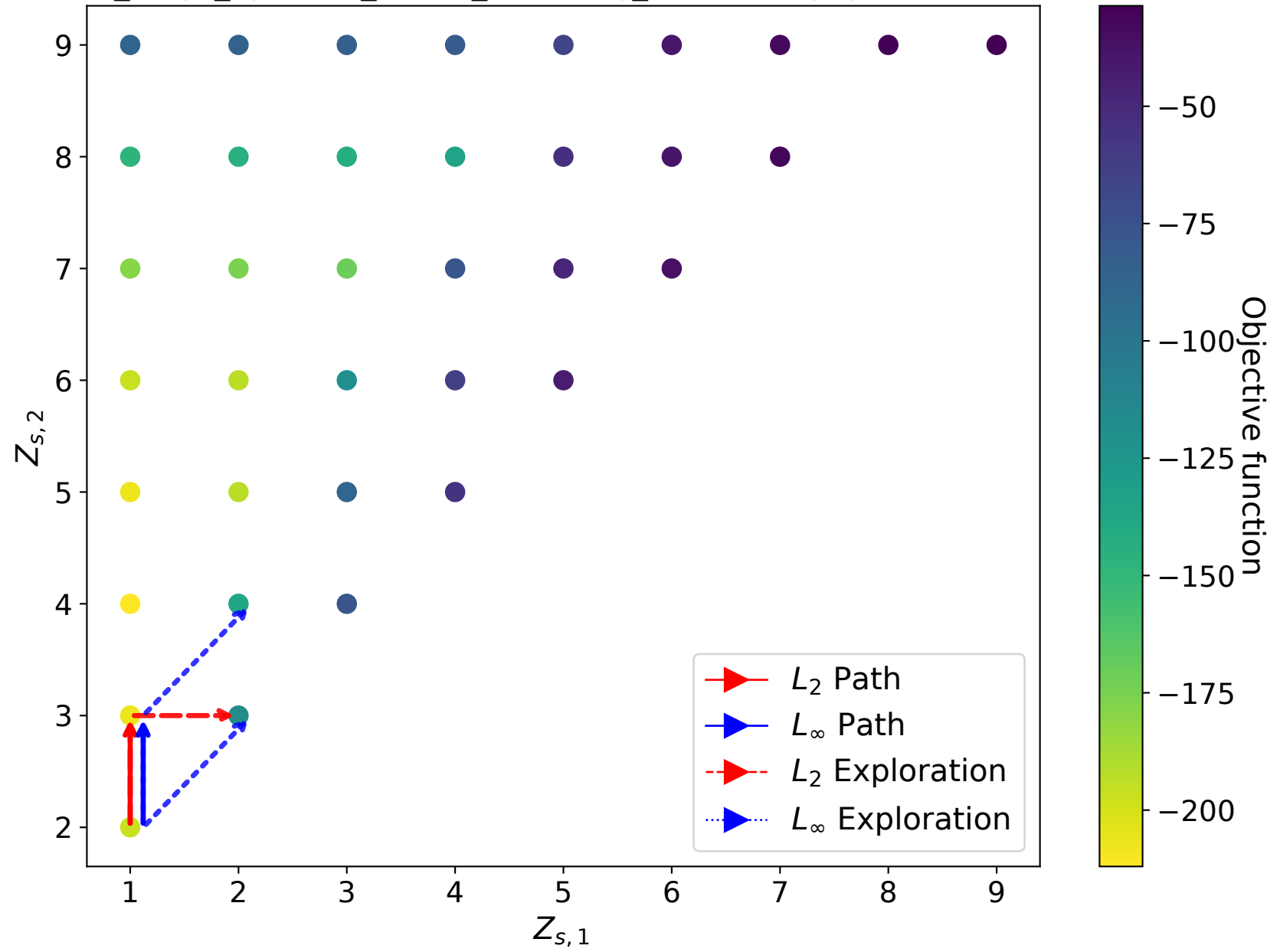
LDSDA nine_stage_dynamic_model_switching_nonlinear ipopt Transfer (L2 vs Linf)
