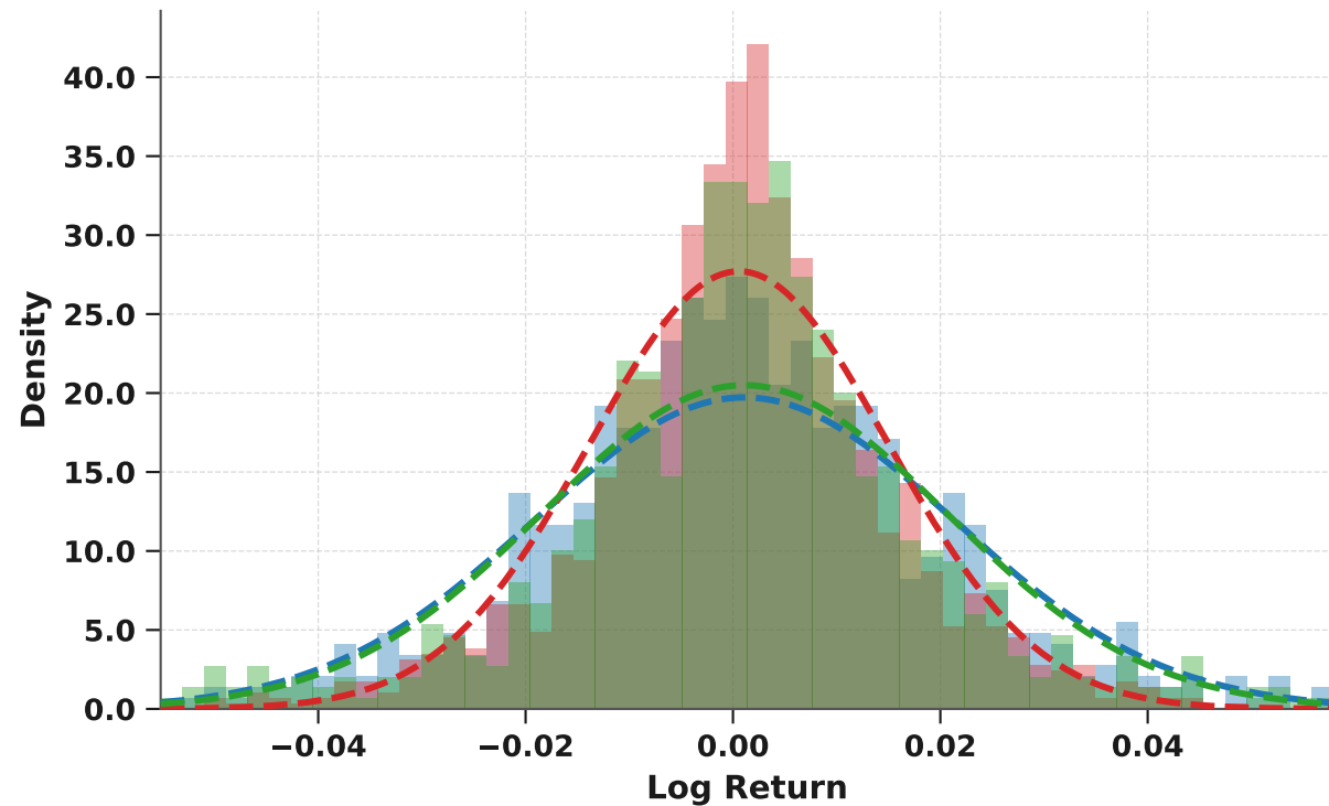
(a) Return Distribution [dashed = fitted Gaussian]
