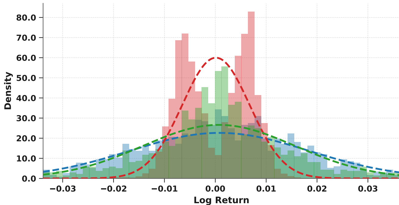
(a) Return Distribution [dashed = fitted Gaussian]
