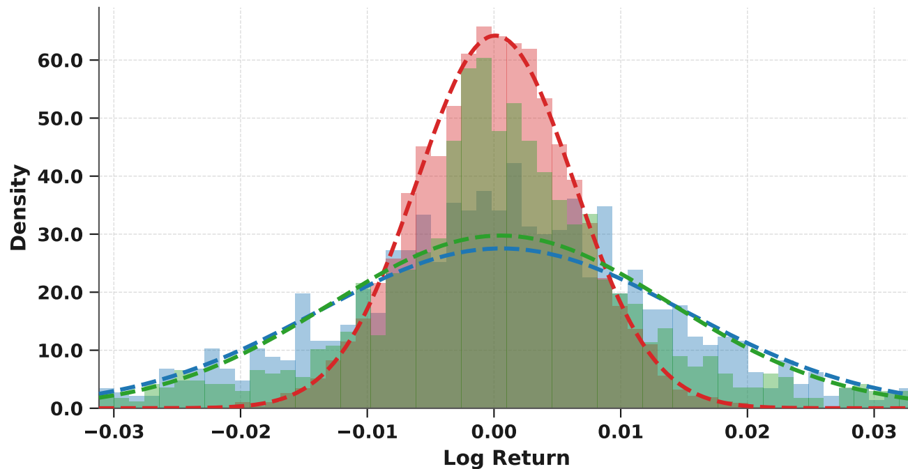
(a) Return Distribution [dashed = fitted Gaussian]
