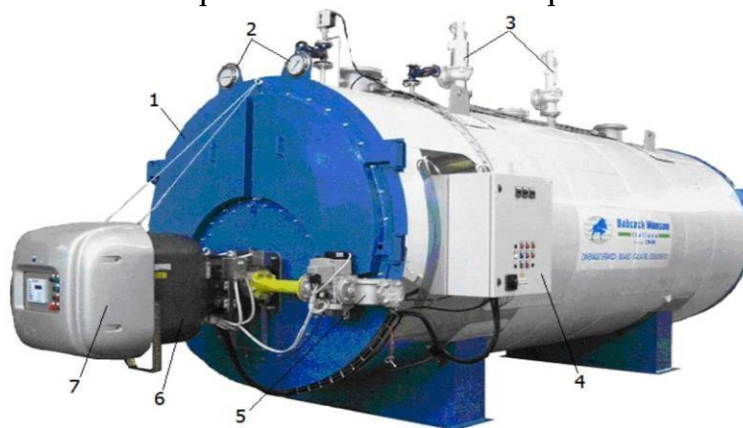
14.2 – rasm. Suv isitish qozoni:
