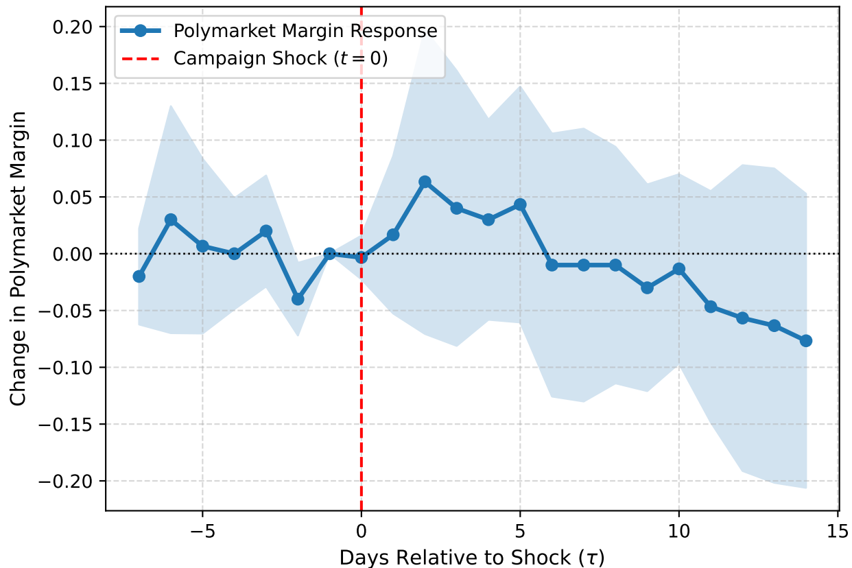
Panel A: Polymarket Odds Response (Instantaneous Jump at t = 0, 1 )
