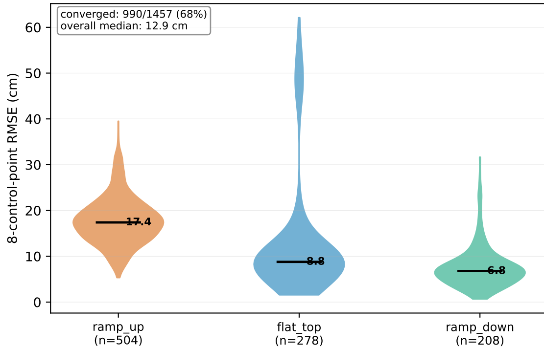
(a) Boundary error by phase
