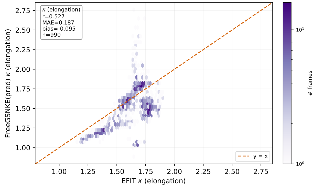
(c) Shape parity
