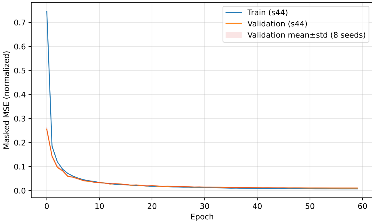
Train / Validation loss (best model: bidir Transformer, time-sinusoidal PE)
