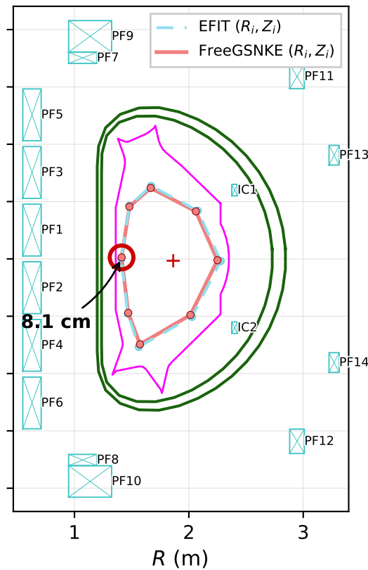
Flat-top @ t=3.85 s
