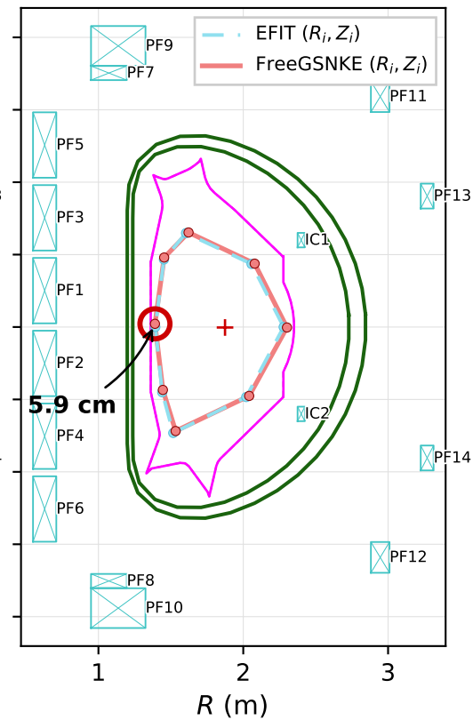
Ramp-down @ t=10.51 s
