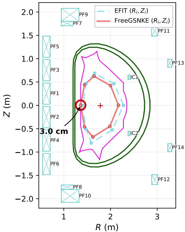
Ramp-up @ t=1.63 s
