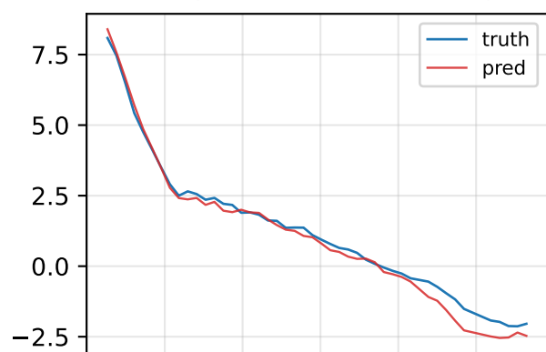
PF1 ( R^2=0.985 , RMSE=0.30 kA)
