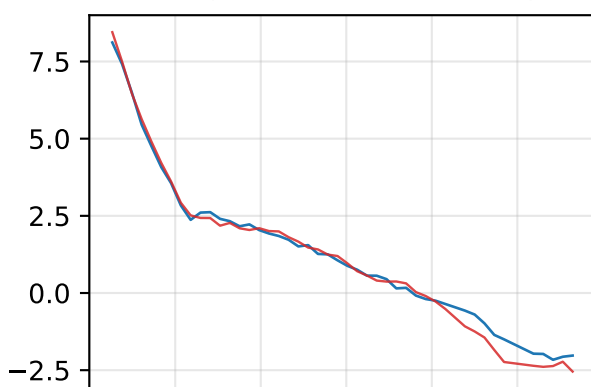
PF2 ( R^2=0.989 , RMSE=0.25 kA)
