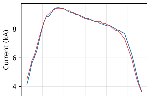
PF7 ( R^2=0.990 , RMSE=0.16 kA)
