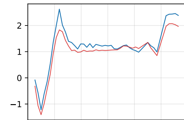
PF13 ( R^2=0.875 , RMSE=0.28 kA)
