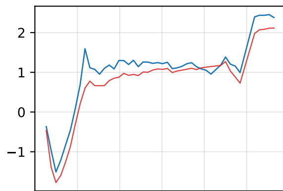
PF14 ( R^2=0.869 , RMSE=0.32 kA)
