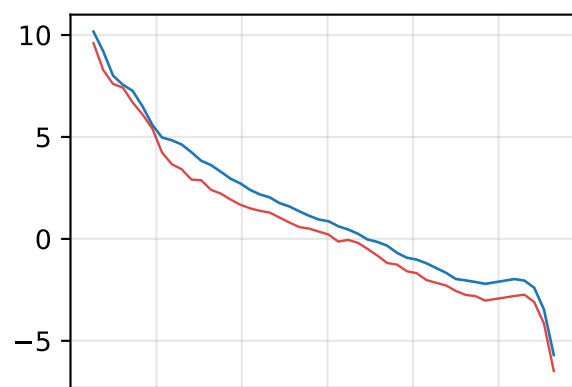
PF6 ( R^2=0.952 , RMSE=0.78 kA)
