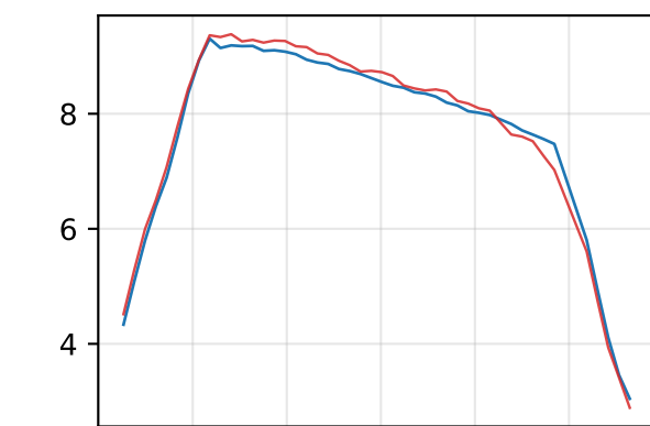
PF8 ( R^2=0.990 , RMSE=0.16 kA)
