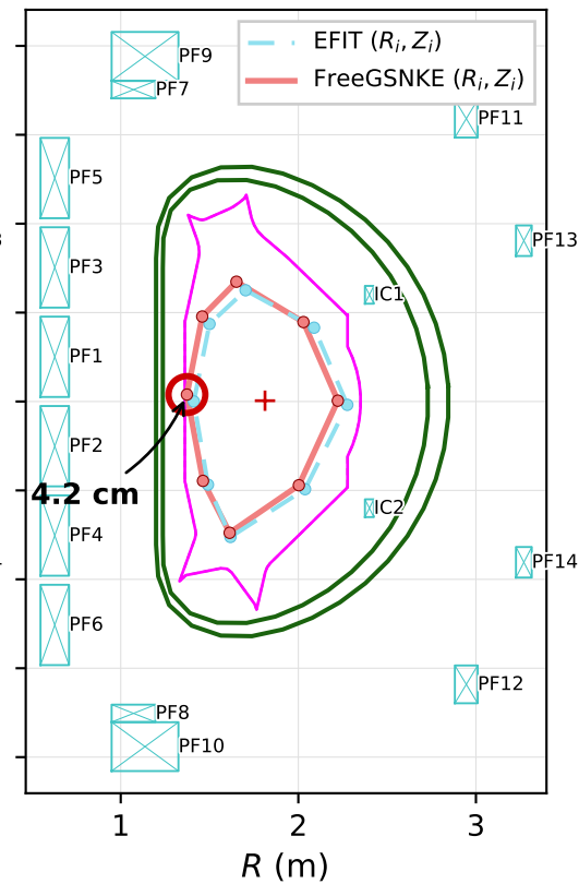
Ramp-down @t=10.38 s
