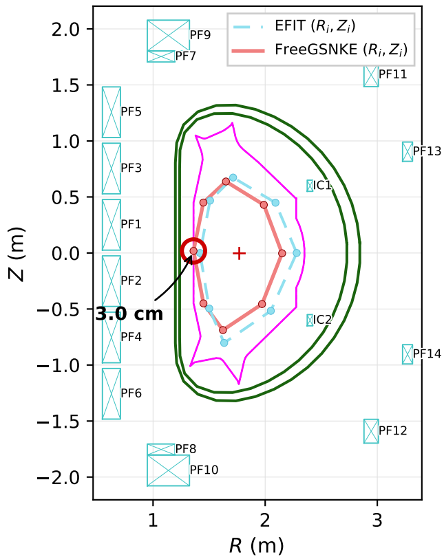
Ramp-up @t=1.90 s
