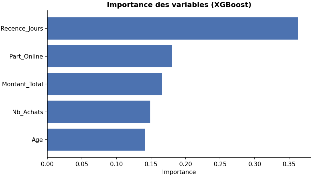
Figure 10 — Importance des variables (XGBoost).
