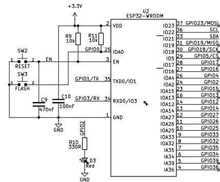
CONTROL & COMMAND
