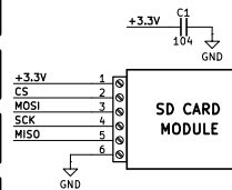
SD CARD MODULE
