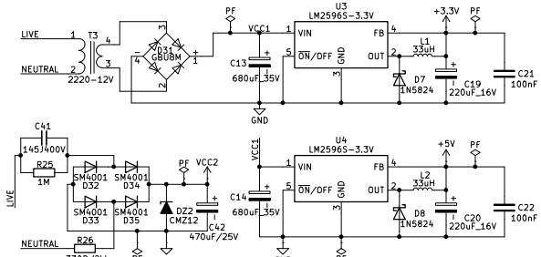
POWER SUPPLY
