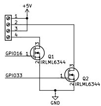
PUMP SYSTEM
