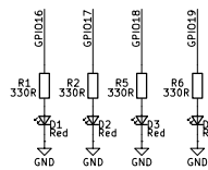
LED INDICATORS
