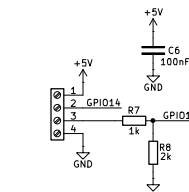
ULTRASONIC SENSOR
