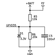
BATTERY LEVEL
