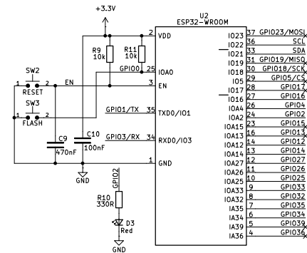
CONTROL & COMMAND
