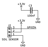
SOIL SENSOR
