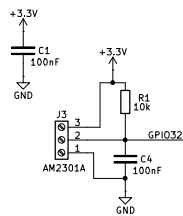
TEMPERATURE & HUMIDITY SENSOR
