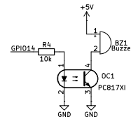
BUZZER
