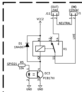
LOAD SWITCHING
