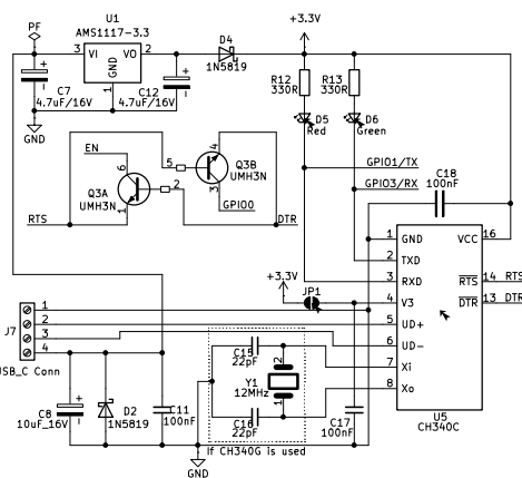
DEBUGGING & PROGRAMMING
