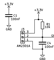
TEMPERATURE SENSOR
