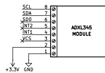
VIBRATION SENSOR
