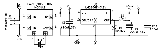
POWER SUPPLY
