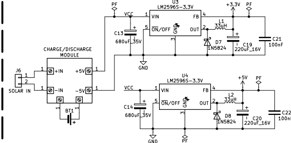
POWER SUPPLY
