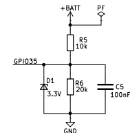
BATTERY LEVEL
