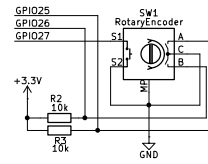
USER INPUT
