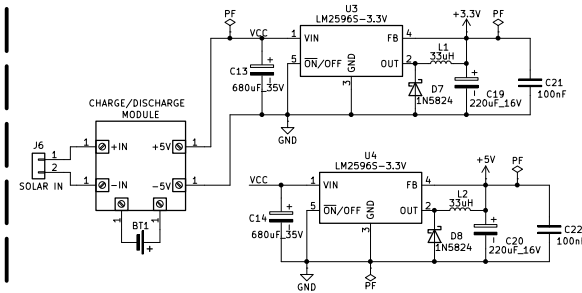
POWER SUPPLY
