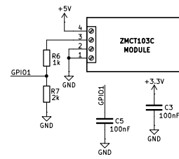
CURRENT SENSOR
