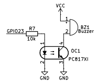
BUZZER
